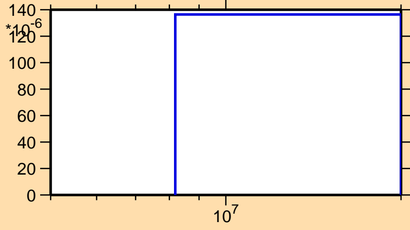
\sigma vs. E for ^{112}\text{Xe}(n,t)
