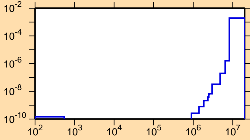
\sigma vs. E for ^{112}\text{Xe}(n,\text{He}3)
