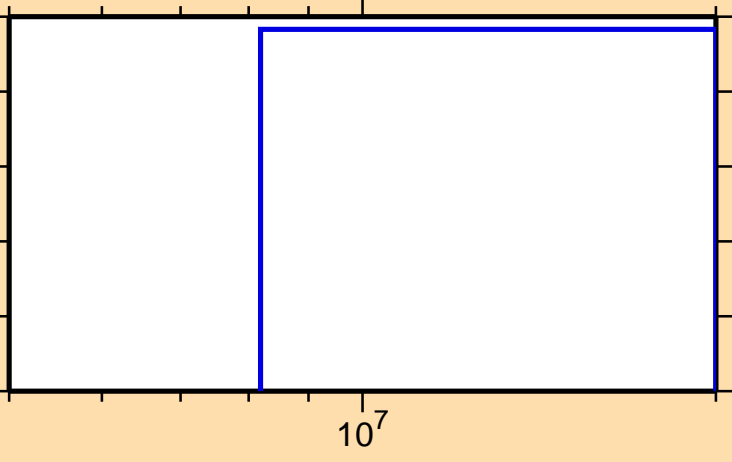
\sigma vs. E for ^{112}\text{Xe}(\text{mt } 34)
