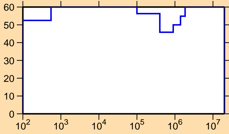
\Delta\sigma/\sigma vs. E for ^{112}\text{Xe}(n,p)
