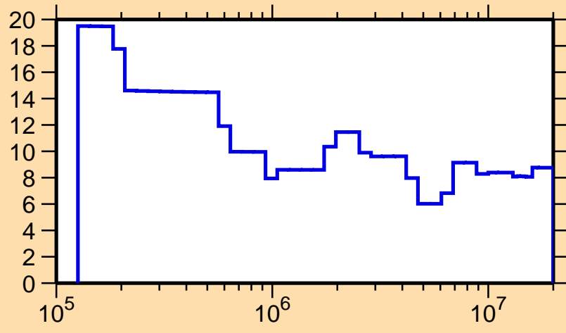
\Delta\sigma/\sigma vs. E for ^{113}\text{Xe}(n,\text{el.})
