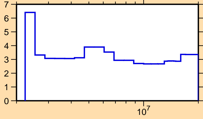
\Delta\sigma/\sigma vs. E for ^{113}\text{Xe}(n,\text{nonel.})
