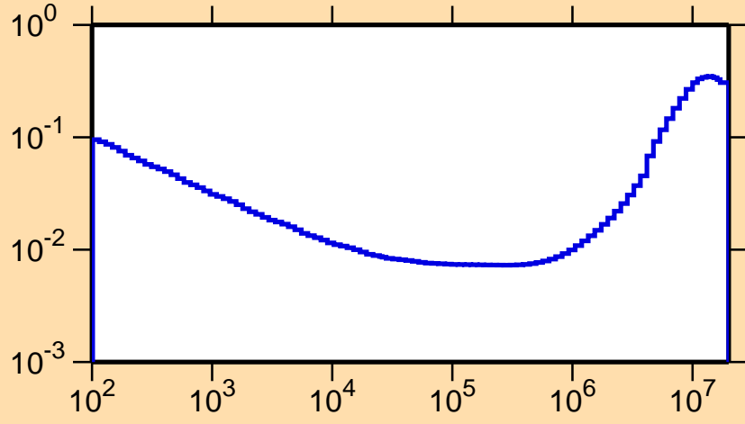
\sigma vs. E for ^{113}\text{Xe}(n,p\alpha)
