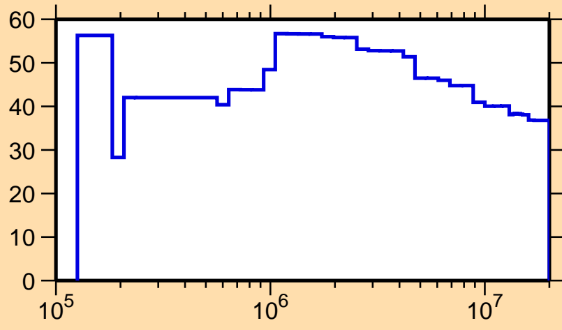
\Delta\sigma/\sigma vs. E for ^{113}\text{Xe}(n,\text{inel.})
