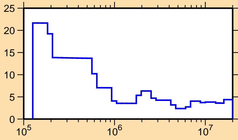
\Delta\sigma/\sigma vs. E for ^{113}\text{Xe}(n,\text{tot.})
