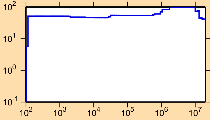
\Delta\sigma/\sigma vs. E for ^{113}\text{Xe}(n,p)
