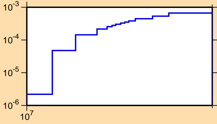
\sigma vs. E for ^{113}\text{Xe}(n,2n)
