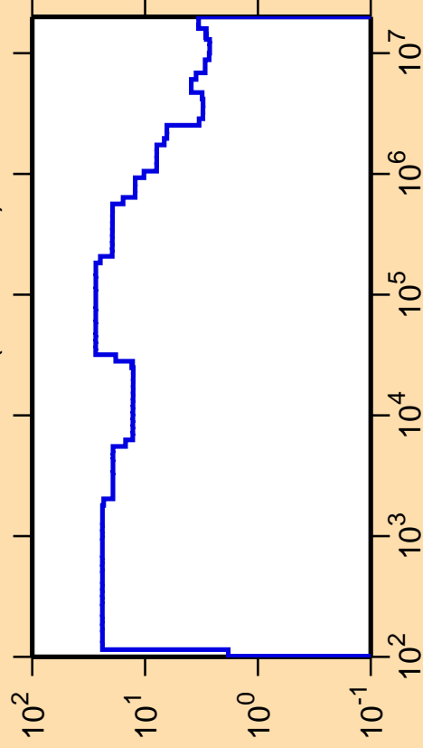
\Delta\sigma/\sigma vs. E for ^{113}\text{Xe}(n,\text{nonel.})
