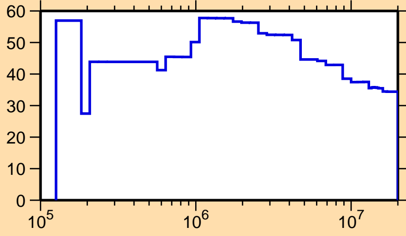
\Delta\sigma/\sigma vs. E for ^{113}\text{Xe}(n,n_1)
