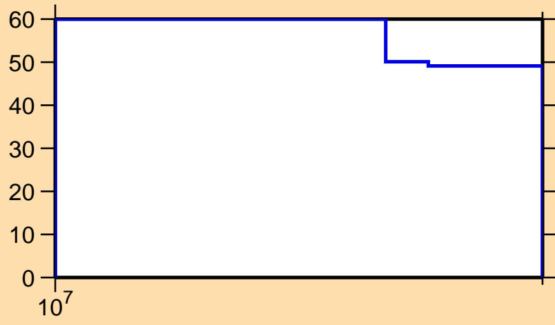
\Delta\sigma/\sigma vs. E for ^{113}\text{Xe}(n,2n)
