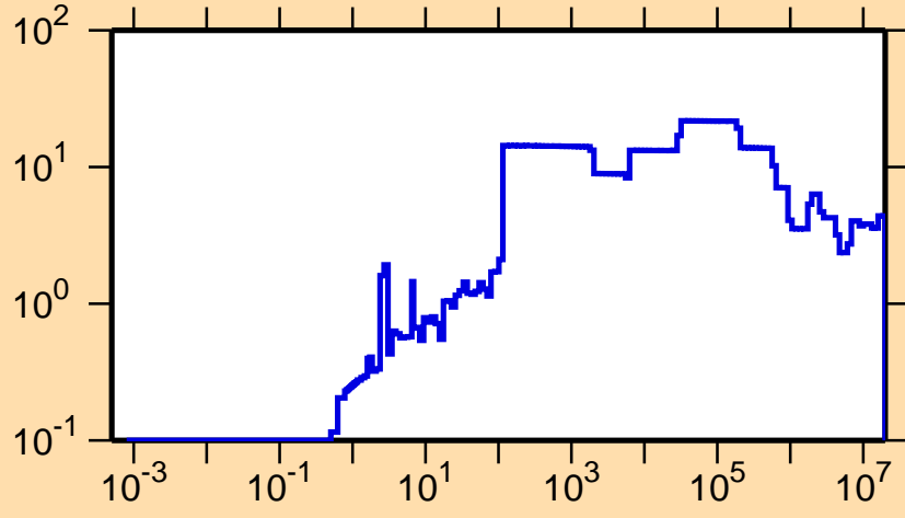
\Delta\sigma/\sigma vs. E for ^{113}\text{Xe}(n,\text{tot.})
