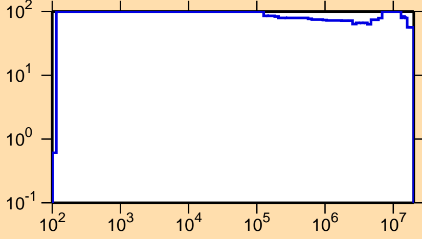
\Delta\sigma/\sigma vs. E for ^{113}\text{Xe}(n,\gamma)
