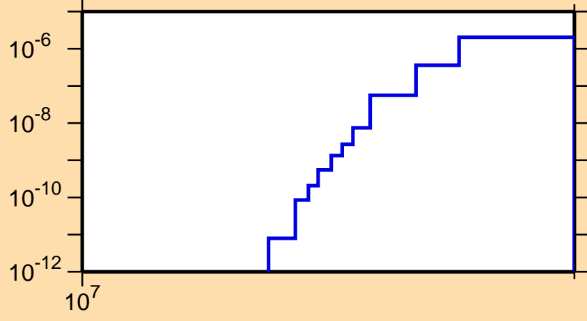
\sigma vs. E for ^{113}\text{Xe}(n,\text{nd})
