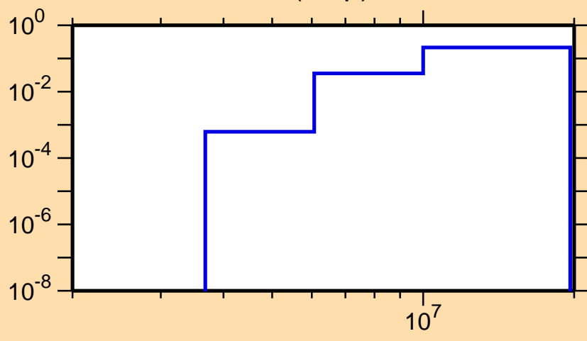
\sigma vs. E for ^{113}\text{Xe}(n,np)
