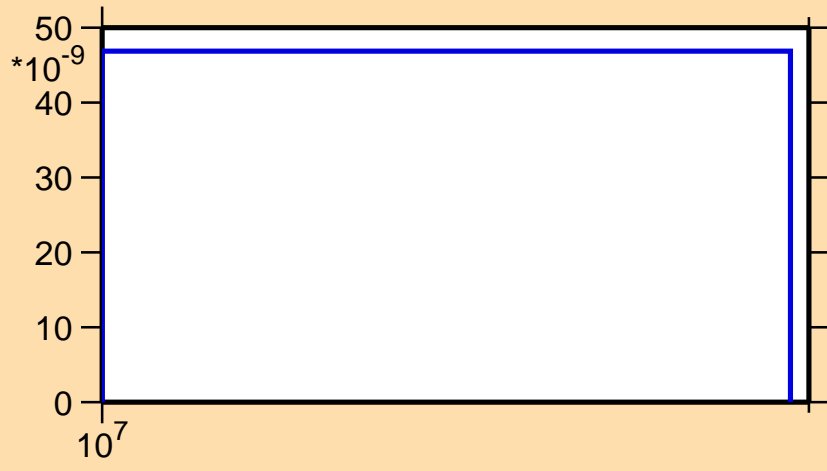
\sigma vs. E for ^{113}\text{Xe}(n,\text{nd})
