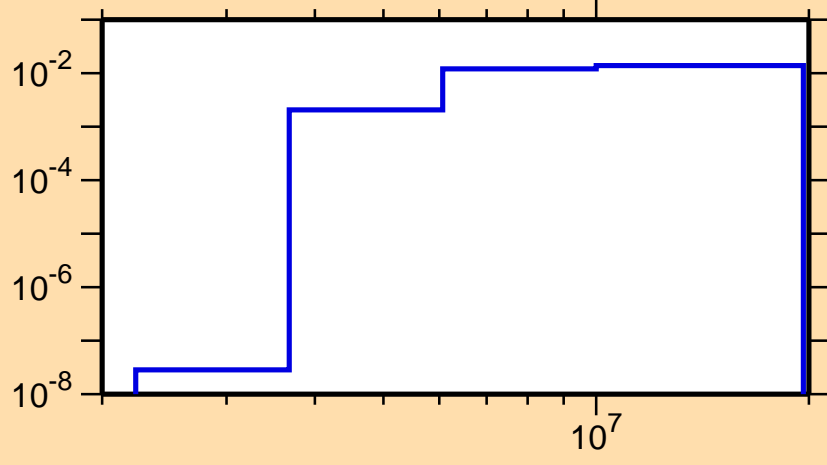
\sigma vs. E for ^{113}\text{Xe}(n,n\text{cont.})
