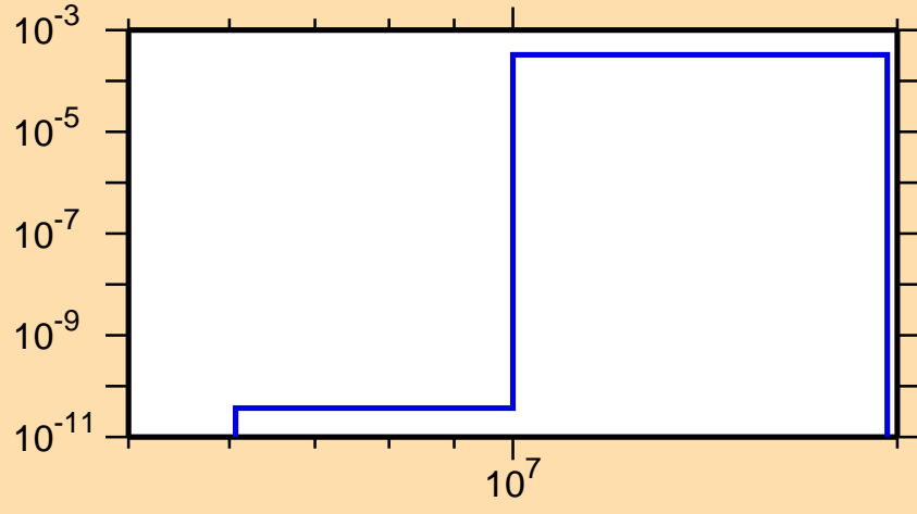
\sigma vs. E for ^{113}\text{Xe}(n,\text{pt})
