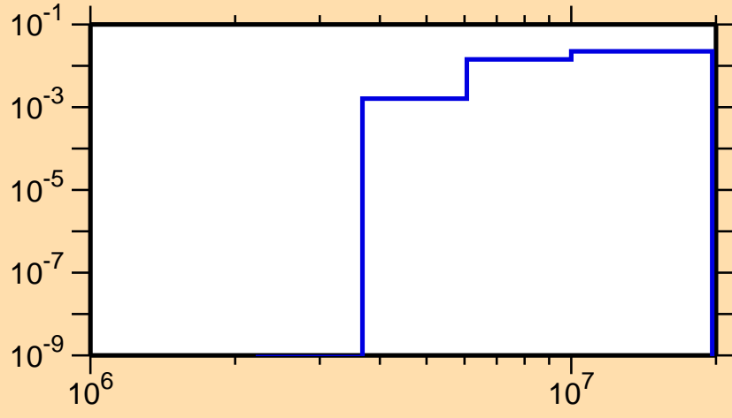
\sigma vs. E for ^{113}\text{Xe}(n,n\alpha)
