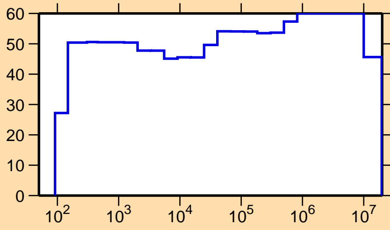
\Delta\sigma/\sigma vs. E for ^{113}\text{Xe}(n,p)
