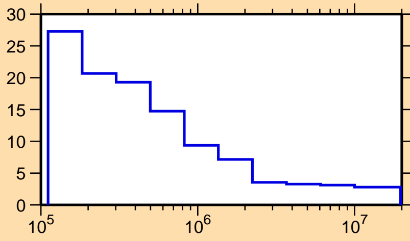
\Delta\sigma/\sigma vs. E for ^{113}\text{Xe}(n,\text{nonel.})
