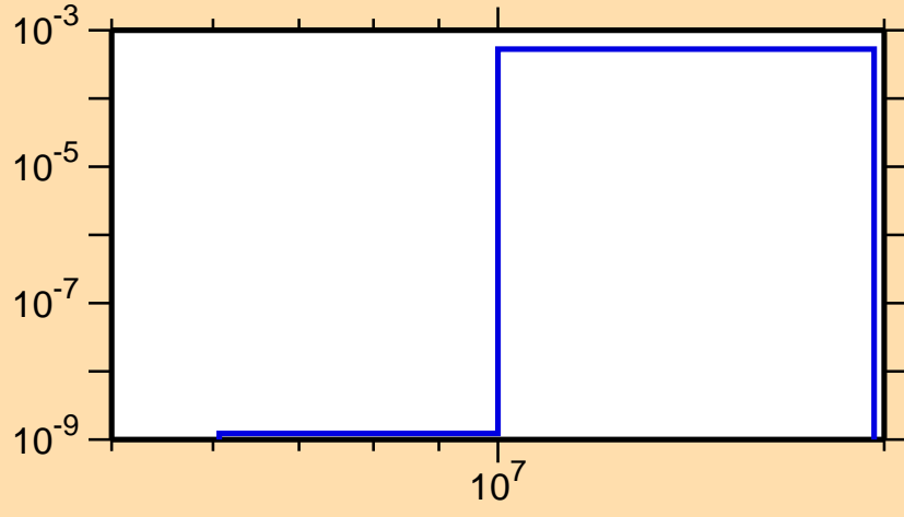
\sigma vs. E for ^{113}\text{Xe}(n,t)
