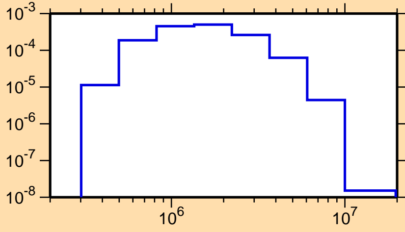
\sigma vs. E for ^{113}\text{Xe}(n,n_3)
