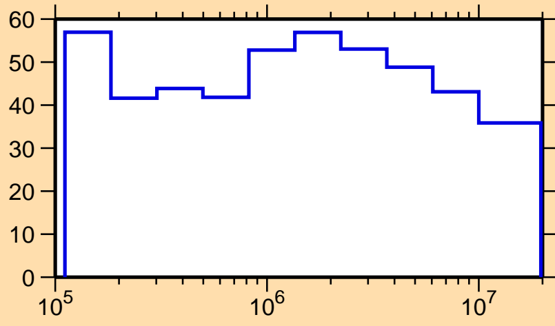
\Delta\sigma/\sigma vs. E for ^{113}\text{Xe}(n,n_1)
