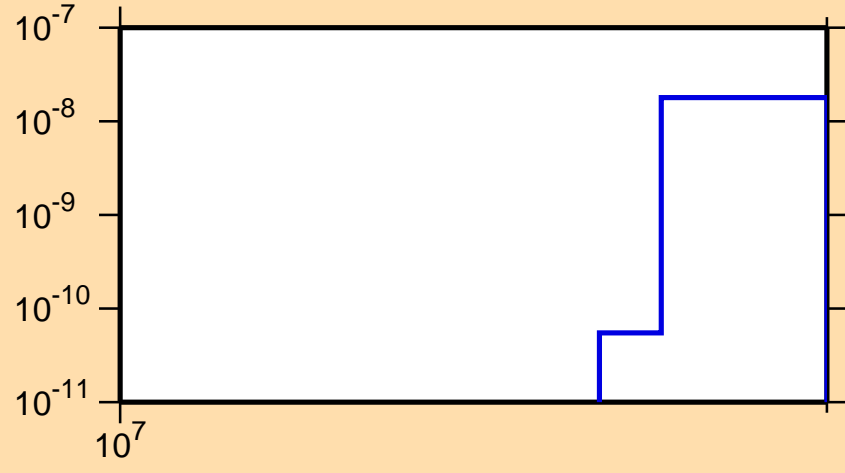
\sigma vs. E for ^{114}\text{Xe}(n,nd)
