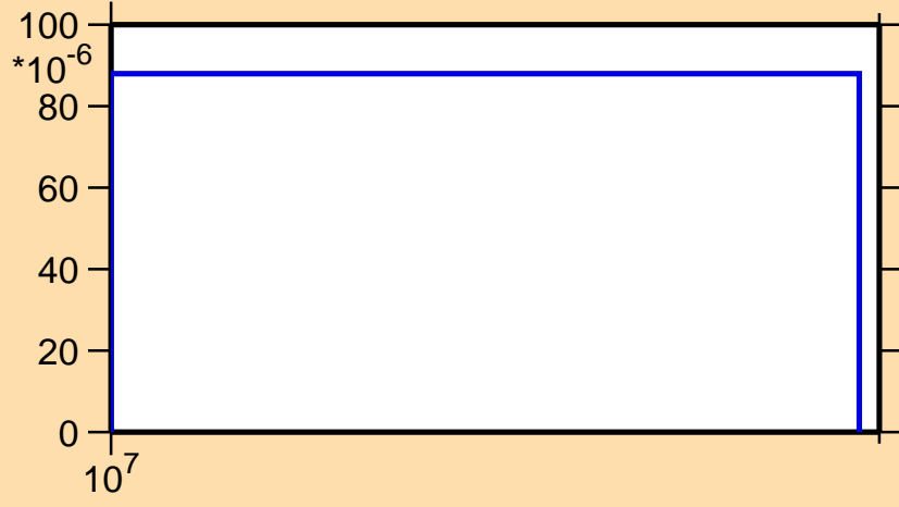
\sigma vs. E for ^{114}\text{Xe}(n,2n)
