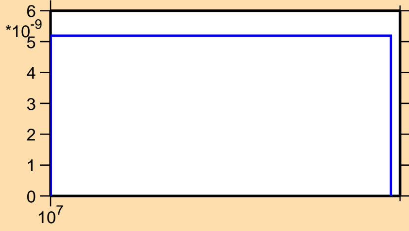
\sigma vs. E for ^{114}\text{Xe}(n,2np)
