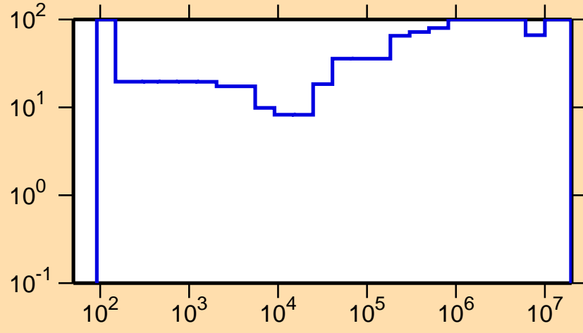
\Delta\sigma/\sigma vs. E for ^{114}\text{Xe}(n,\gamma)
