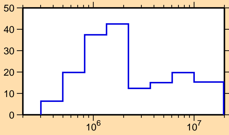
\Delta\sigma/\sigma vs. E for ^{114}\text{Xe}(n,\text{el.})
