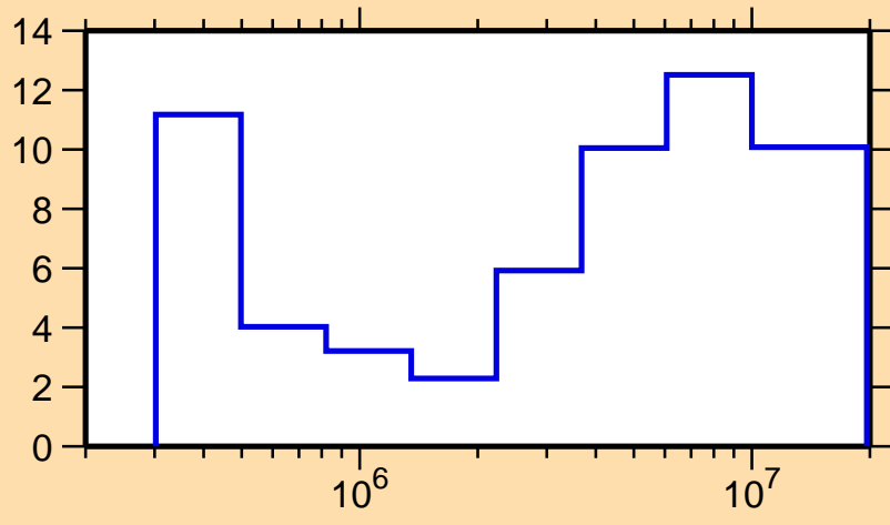
\Delta\sigma/\sigma vs. E for ^{114}\text{Xe}(n,\text{nonel.})
