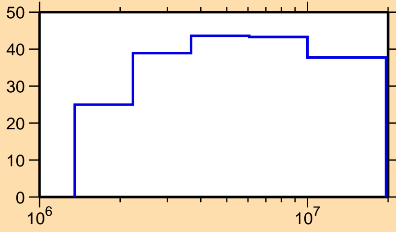
\Delta\sigma/\sigma vs. E for ^{114}\text{Xe}(n,n_1)
