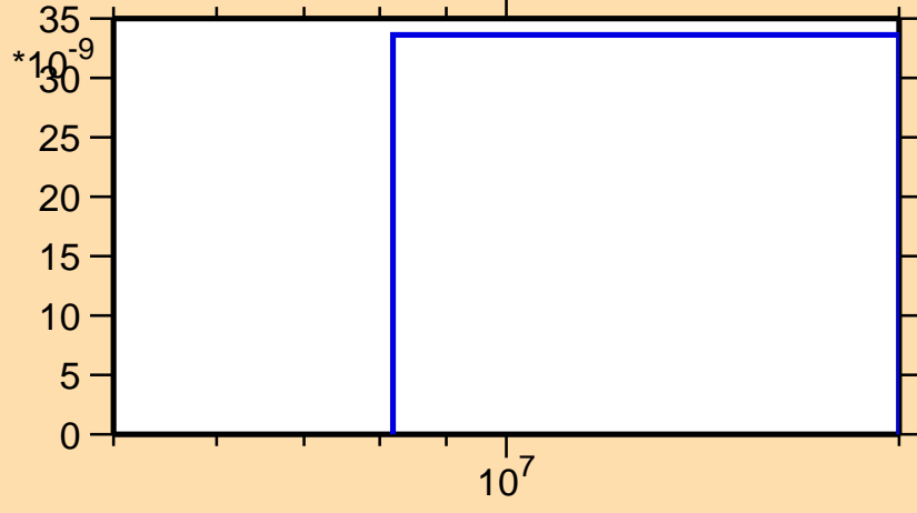
\sigma vs. E for ^{114}\text{Xe}(n,2n\alpha)
