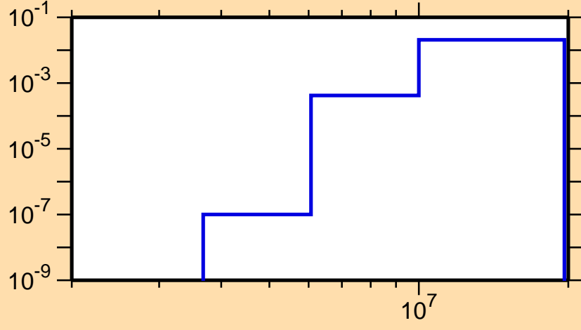
\sigma vs. E for ^{115}\text{Xe}(n,d)
