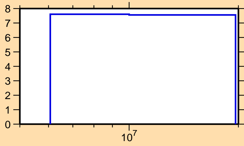
\Delta\sigma/\sigma vs. E for ^{115}\text{Xe}(n,\text{el.})
