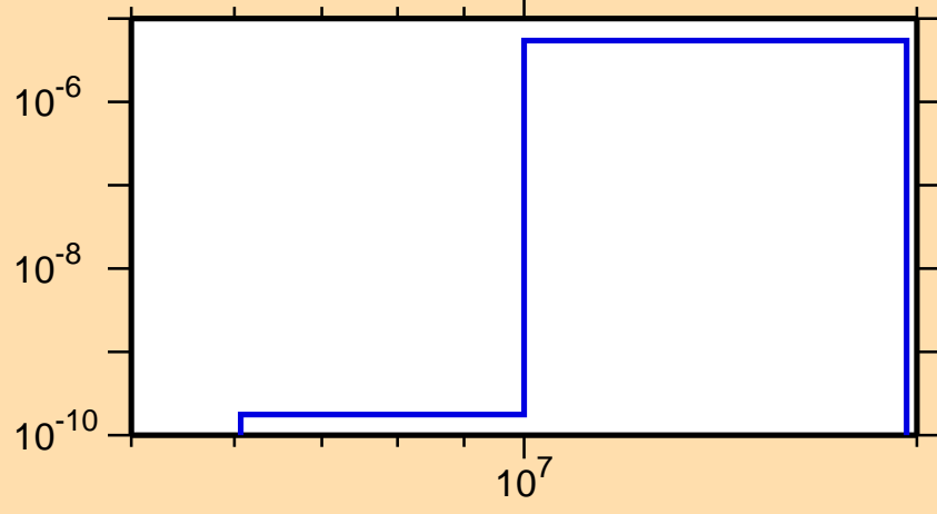
\sigma vs. E for ^{115}\text{Xe}(\text{mt117})
