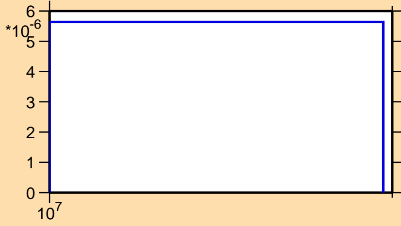
\sigma vs. E for ^{115}\text{Xe}(n,2np)
