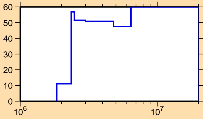
\Delta\sigma/\sigma vs. E for ^{115}\text{Xe}(n,n\text{cont.})
