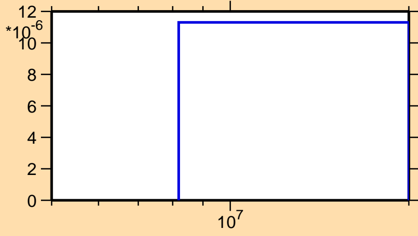
\sigma vs. E for ^{115}\text{Xe}(n,2n\alpha)
