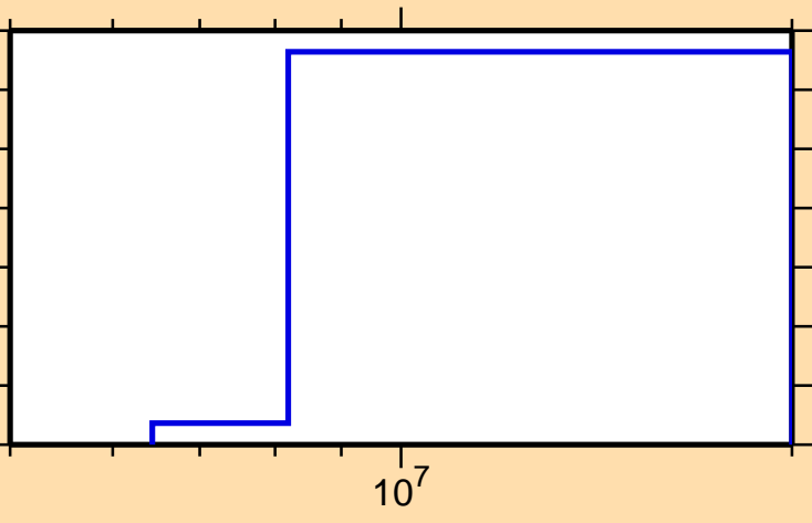
\sigma vs. E for ^{115}\text{Xe}(\text{mt117})
