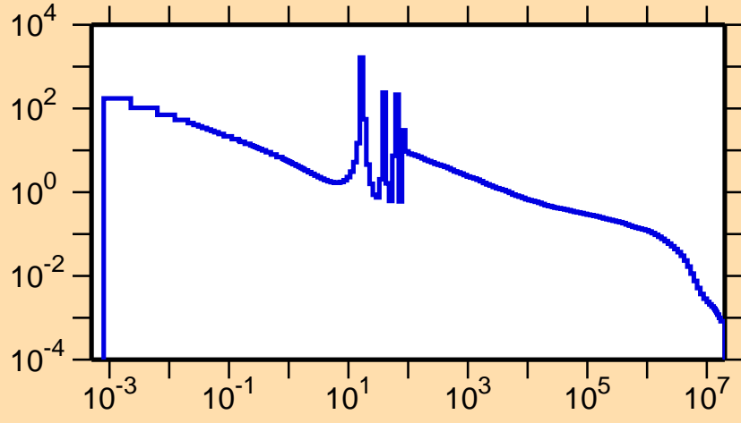
\sigma vs. E for ^{116}\text{Xe}(n,\gamma)
