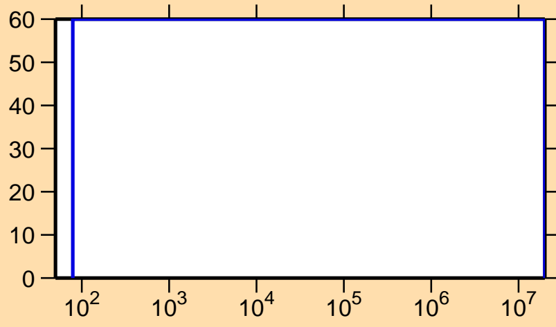
\Delta\sigma/\sigma vs. E for ^{116}\text{Xe}(n,\gamma)
