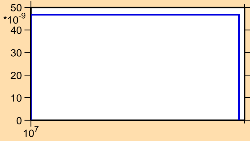
\sigma vs. E for ^{116}\text{Xe}(n,2n\alpha)
