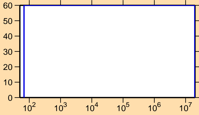
\Delta\sigma/\sigma vs. E for ^{116}\text{Xe}(n,\gamma)
