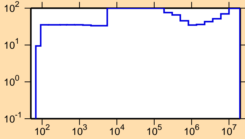
\Delta\sigma/\sigma vs. E for ^{116}\text{Xe}(n,p)
