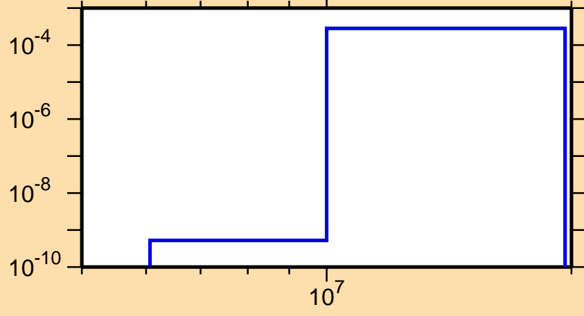
\sigma vs. E for ^{116}\text{Xe}(n,\text{pd})
