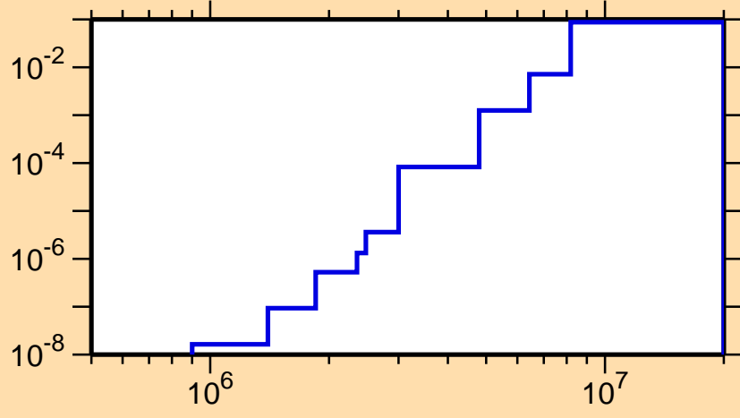
\sigma vs. E for ^{116}\text{Xe}(n,p\alpha)
