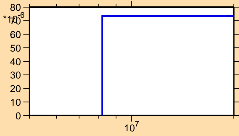
\sigma vs. E for ^{116}\text{Xe}(n,t)
