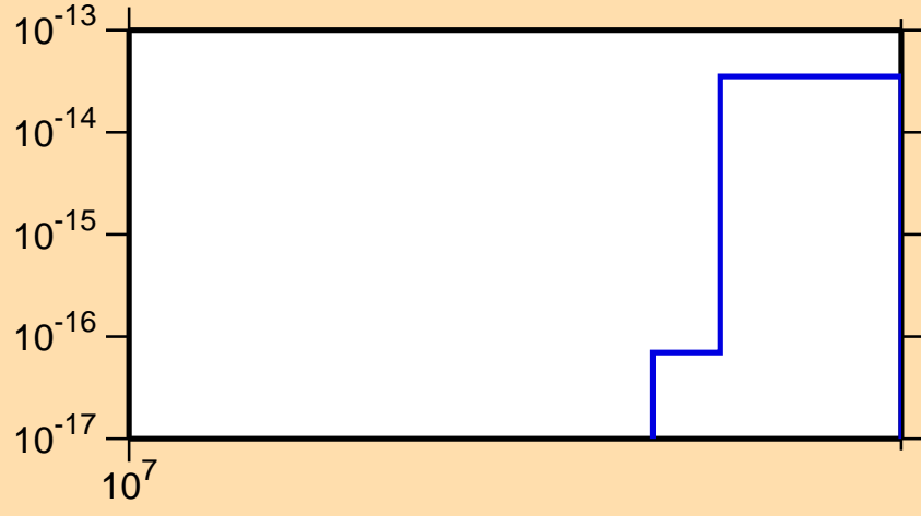
\sigma vs. E for ^{117}\text{Xe}(n,nt)
