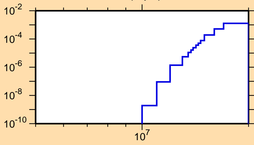
\sigma vs. E for ^{117}\text{Xe}(n,\text{pd})
