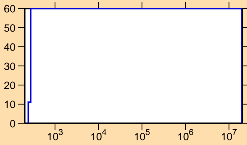
\Delta\sigma/\sigma vs. E for ^{117}\text{Xe}(n,\gamma)
