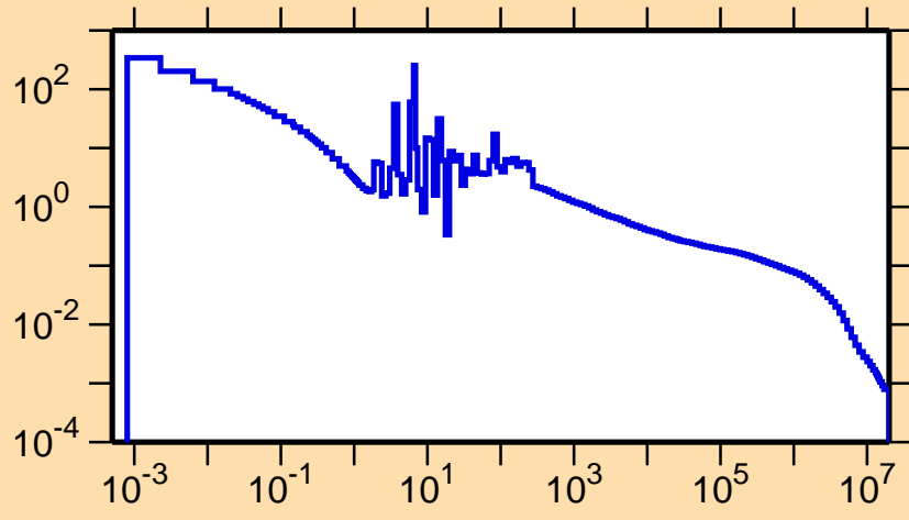
\sigma vs. E for ^{117}\text{Xe}(n,\gamma)
