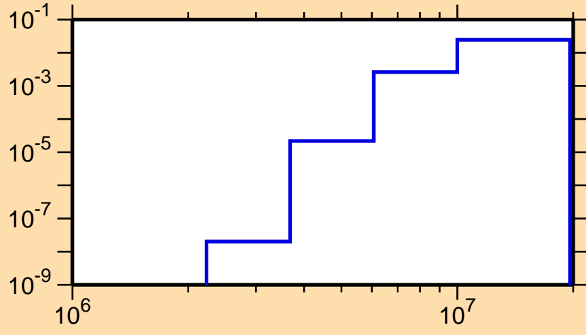
\sigma vs. E for ^{117}\text{Xe}(n,n\alpha)
