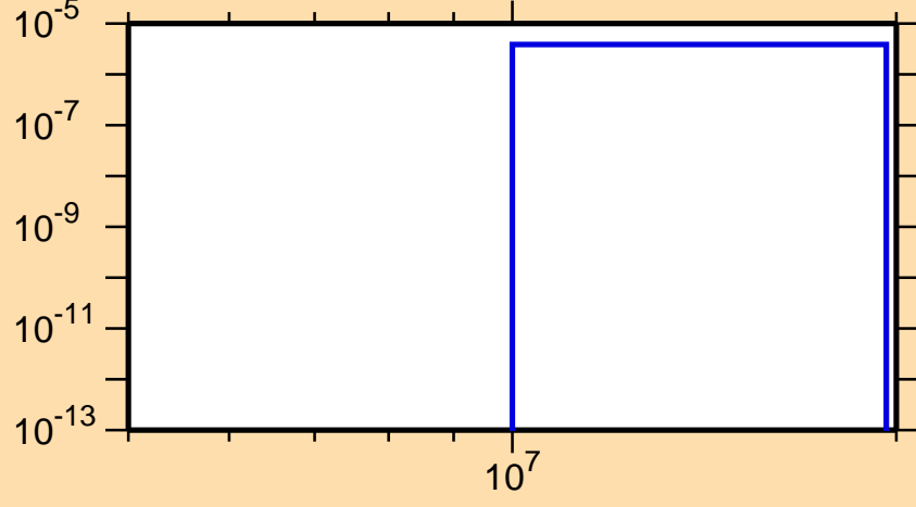
\sigma vs. E for ^{117}\text{Xe}(n,pt)
