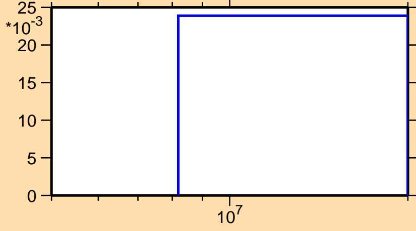
\sigma vs. E for ^{117}\text{Xe}(n,2n)
