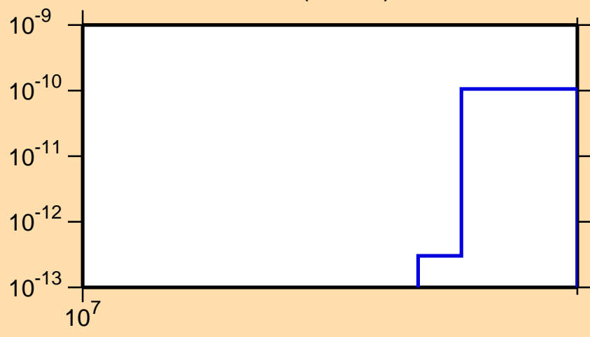
\sigma vs. E for ^{118}\text{Xe}(\text{mt } 34)
