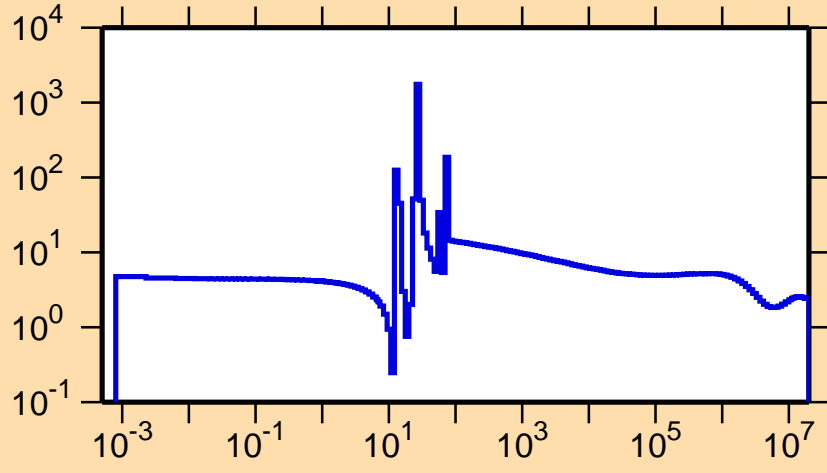
\sigma vs. E for ^{118}\text{Xe}(n,\text{el.})
