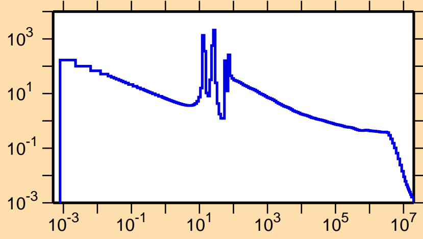
\sigma vs. E for ^{118}\text{Xe}(n,\gamma)
