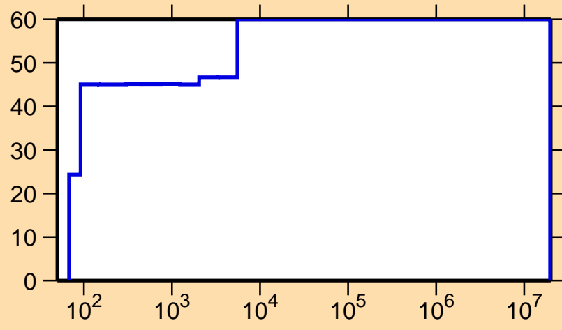
\Delta\sigma/\sigma vs. E for ^{118}\text{Xe}(n,\gamma)
