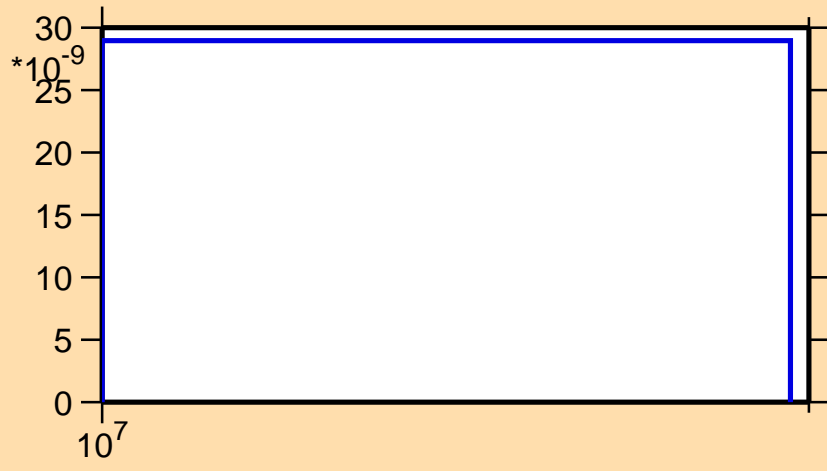
\sigma vs. E for ^{118}\text{Xe}(n,2n\alpha)
