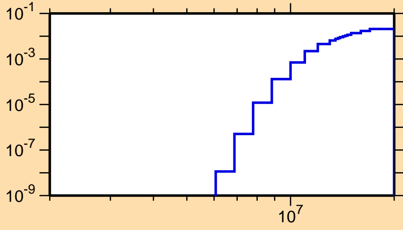
\sigma vs. E for ^{119}\text{Xe}(n,d)
