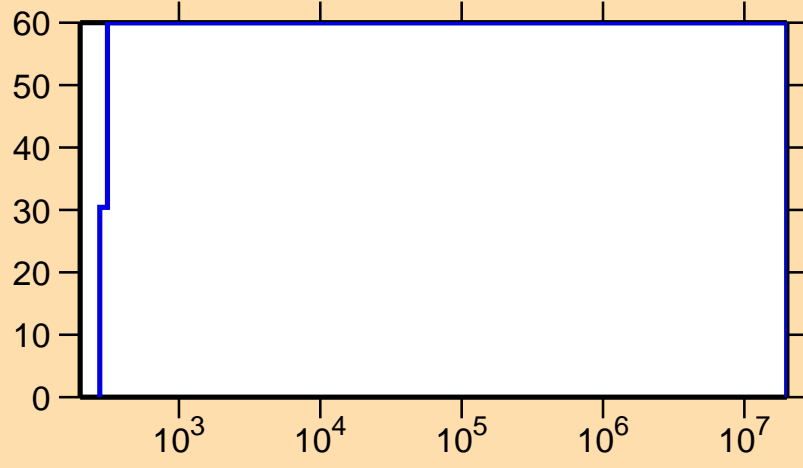
\Delta\sigma/\sigma vs. E for ^{119}\text{Xe}(n,\gamma)
