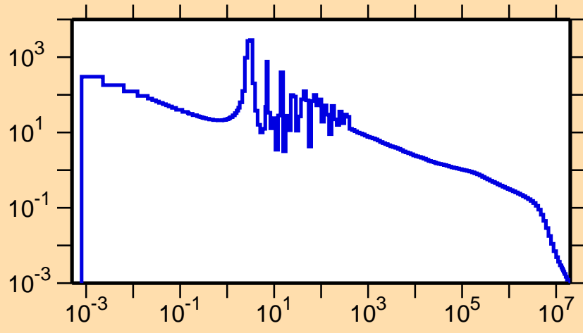
\sigma vs. E for ^{119}\text{Xe}(n,\gamma)
