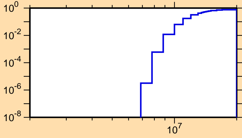
\sigma vs. E for ^{119}\text{Xe}(n,np)
