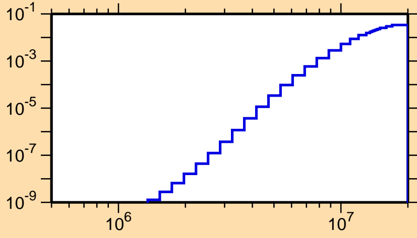
\sigma vs. E for ^{119}\text{Xe}(n,p\alpha)
