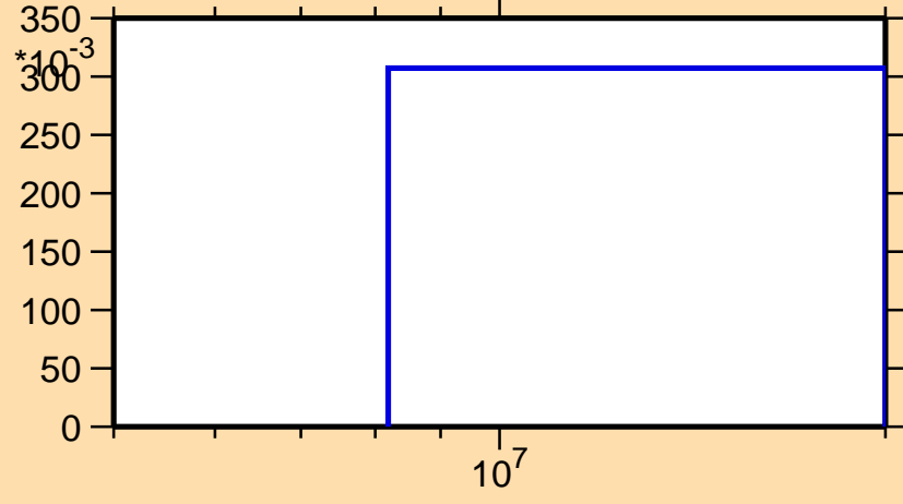
\sigma vs. E for ^{119}\text{Xe}(n,2n)
