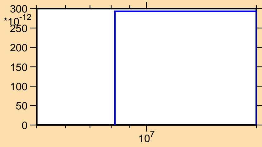
\sigma vs. E for ^{120}\text{Xe}(n,nd)
