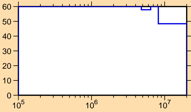
\Delta\sigma/\sigma vs. E for ^{120}\text{Xe}(n,n_1)
