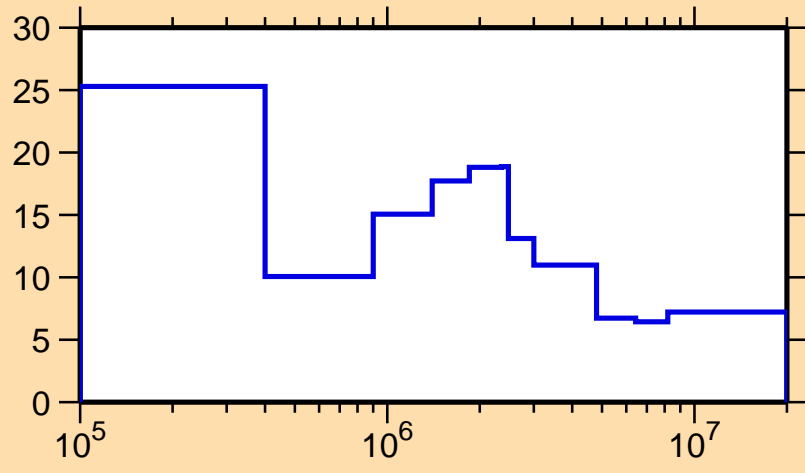
\Delta\sigma/\sigma vs. E for ^{120}\text{Xe}(n,\text{tot.})
