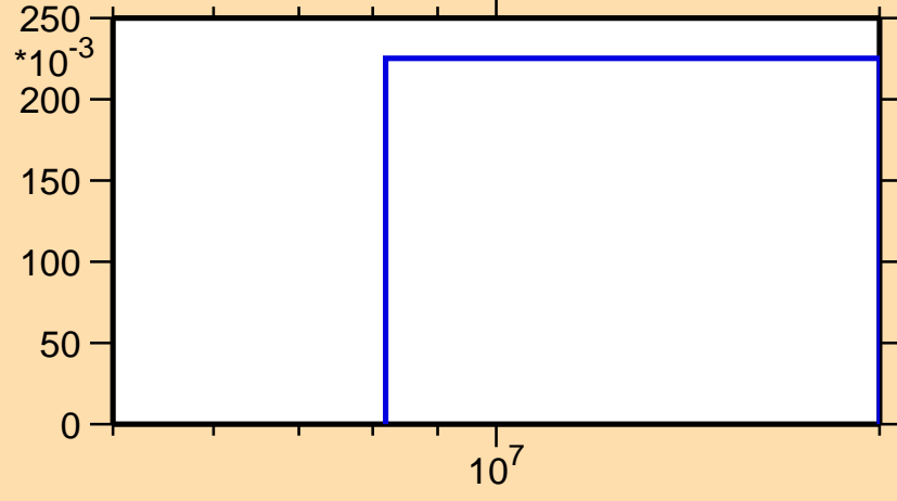
\sigma vs. E for ^{120}\text{Xe}(n,2n)
