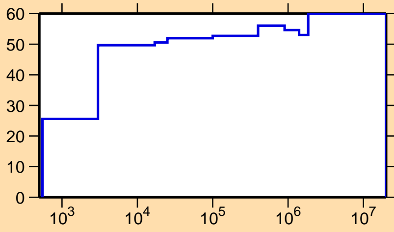
\Delta\sigma/\sigma vs. E for ^{120}\text{Xe}(n,\gamma)
