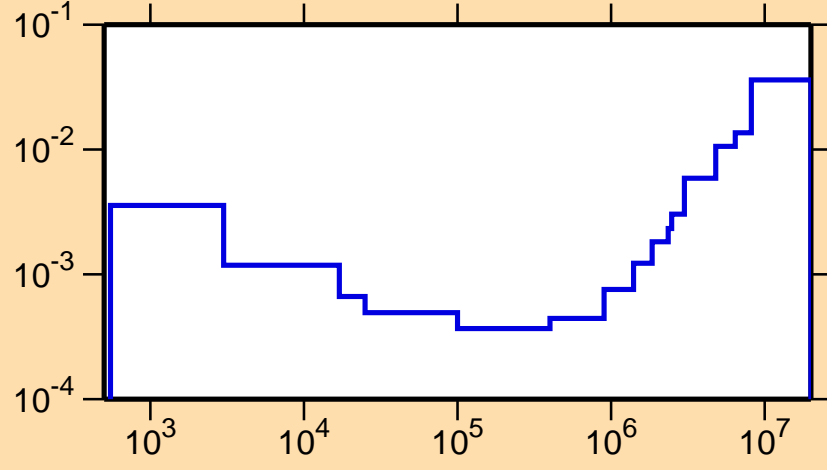
\sigma vs. E for ^{120}\text{Xe}(n,\alpha)
