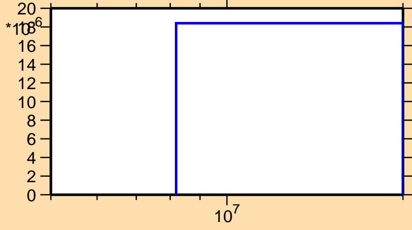
\sigma vs. E for ^{120}\text{Xe}(n,t)
