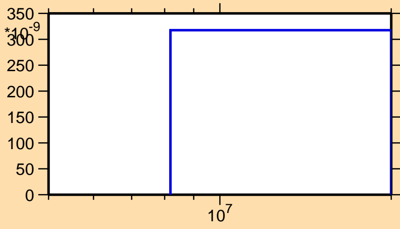
\sigma vs. E for ^{120}\text{Xe}(n,\text{pd})
