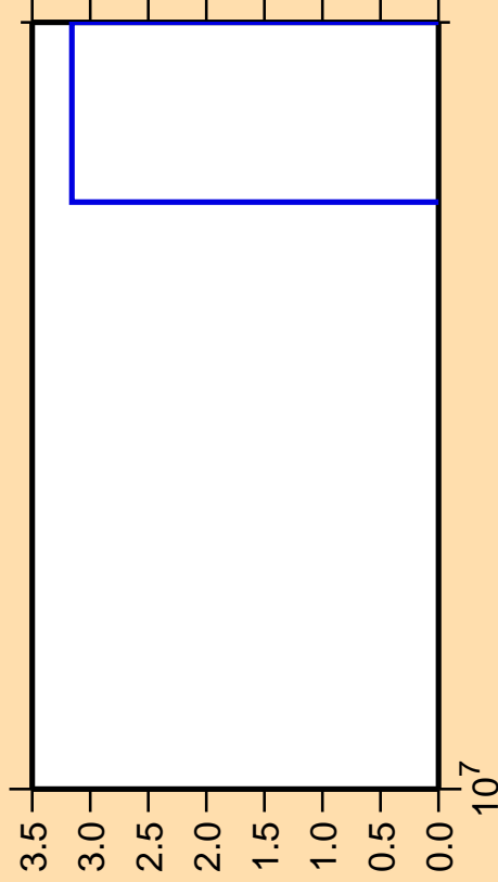
\Delta\sigma/\sigma vs. E for ^{121}\text{Xe}(n,3n)
