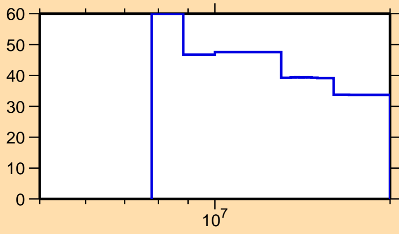
\Delta\sigma/\sigma vs. E for ^{121}\text{Xe}(n,2n)
