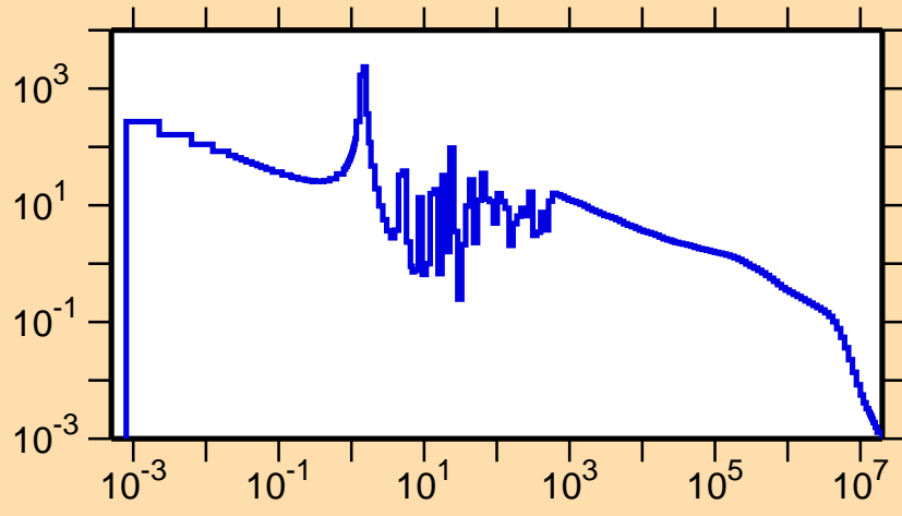
\sigma vs. E for ^{121}\text{Xe}(n,\gamma)
