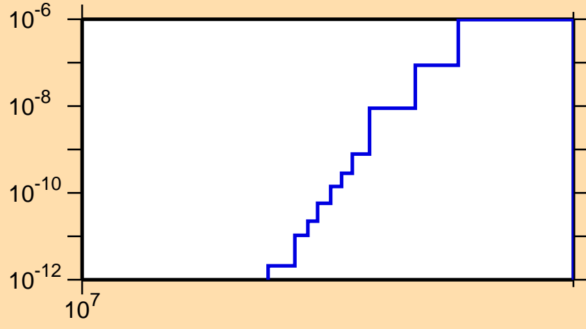
\sigma vs. E for ^{121}\text{Xe}(\text{mt } 45)
