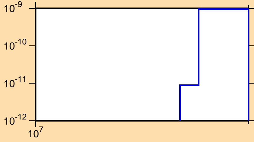
\sigma vs. E for ^{121}\text{Xe} (mt 34)
