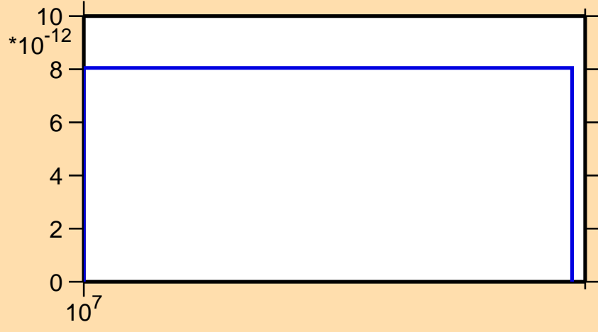
\sigma vs. E for ^{121}\text{Xe} (mt 34)
