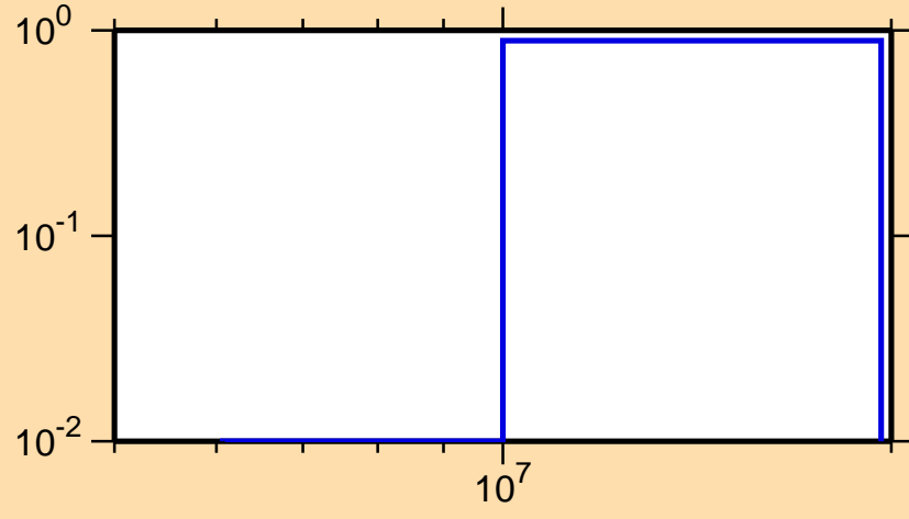
\sigma vs. E for ^{121}\text{Xe}(n,2n)
