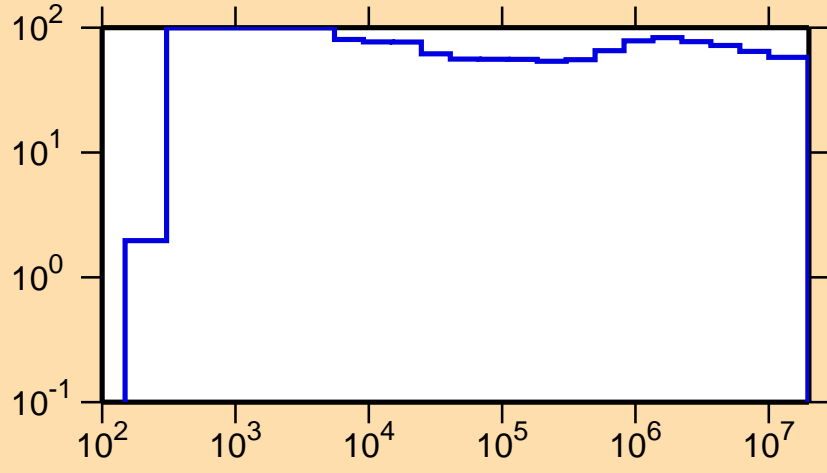
\Delta\sigma/\sigma vs. E for ^{121}\text{Xe}(n,p)
