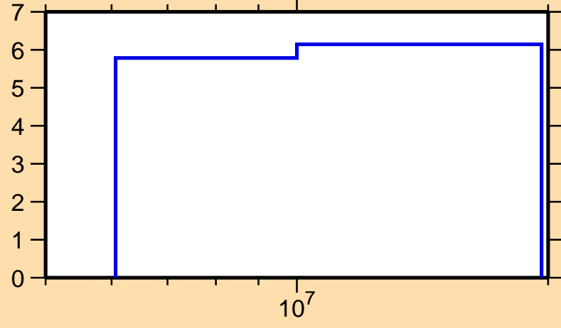
\Delta\sigma/\sigma vs. E for ^{121}\text{Xe}(n,\text{nonel.})
