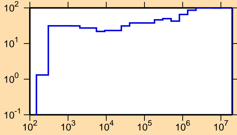
\Delta\sigma/\sigma vs. E for ^{121}\text{Xe}(n,\gamma)
