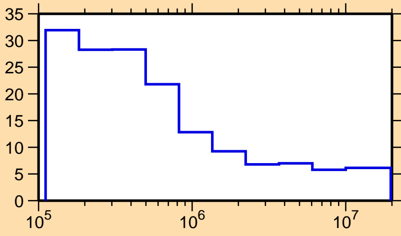
\Delta\sigma/\sigma vs. E for ^{121}\text{Xe}(n,\text{nonel.})
