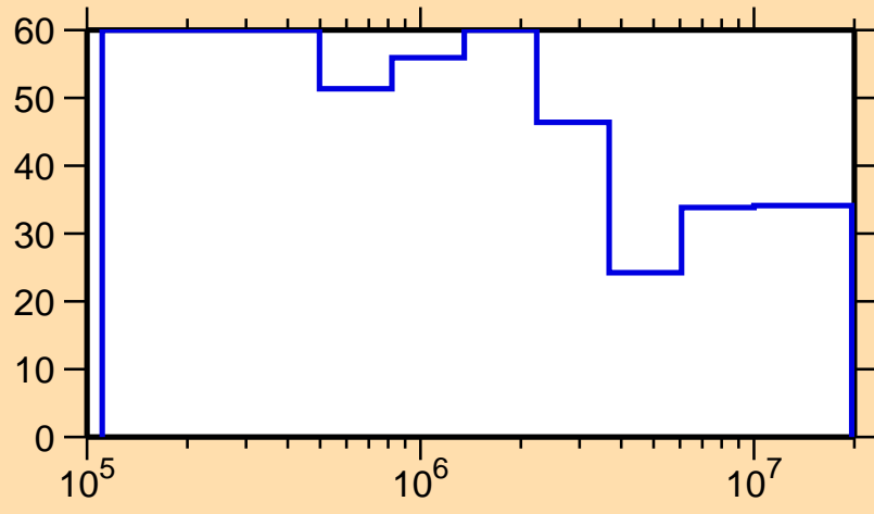
\Delta\sigma/\sigma vs. E for ^{121}\text{Xe}(n,n_1)
