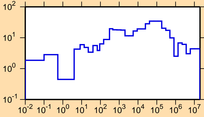
\Delta\sigma/\sigma vs. E for ^{121}\text{Xe}(n,\text{tot.})
