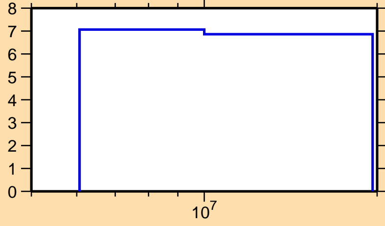
\Delta\sigma/\sigma vs. E for ^{121}\text{Xe}(n,\text{el.})
