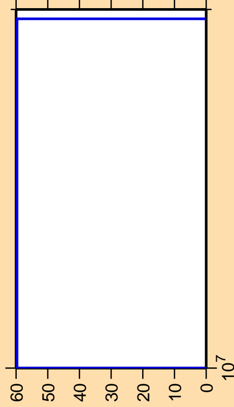
\Delta\sigma/\sigma vs. E for ^{121}\text{Xe} (mt 34)
