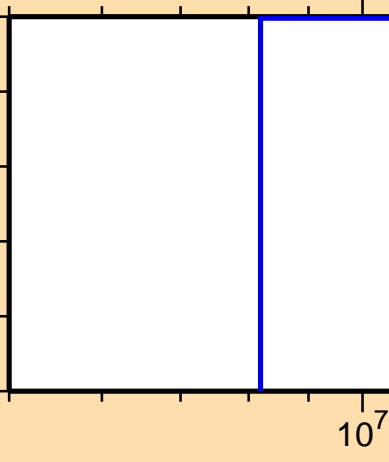
\sigma vs. E for ^{121}\text{Xe}(n,\text{He}3)
