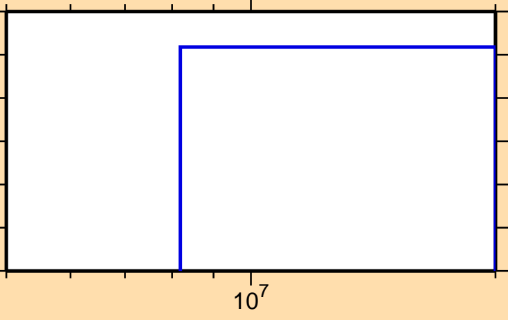
\sigma vs. E for ^{121}\text{Xe}(n,3n)
