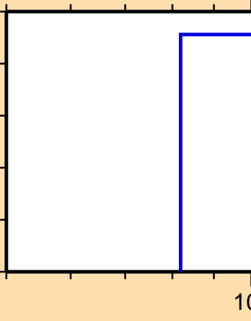
\sigma vs. E for ^{121}\text{Xe}(n,2n\alpha)
