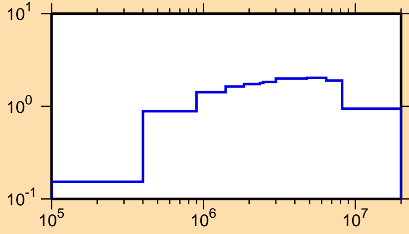
\sigma vs. E for ^{121}\text{Xe}(n,\text{inel.})
