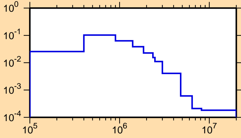
\sigma vs. E for ^{121}\text{Xe}(n,n_4)
