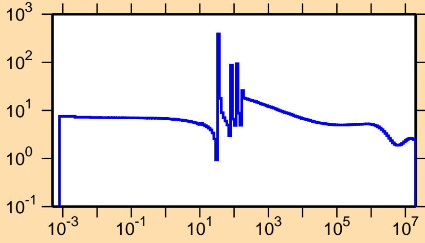
\sigma vs. E for ^{122}\text{Xe}(n,\text{el.})
