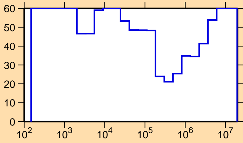
\Delta\sigma/\sigma vs. E for ^{122}\text{Xe}(n,\gamma)
