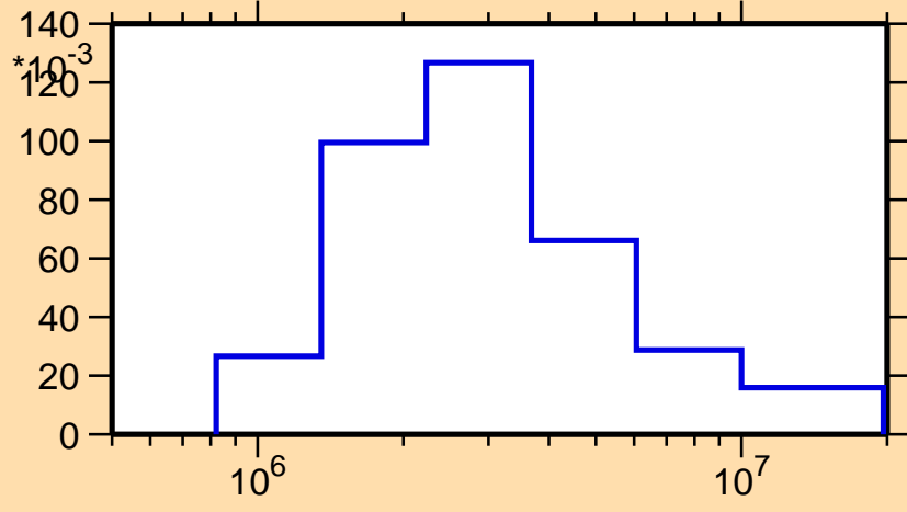
\sigma vs. E for ^{122}\text{Xe}(n,n_2)
