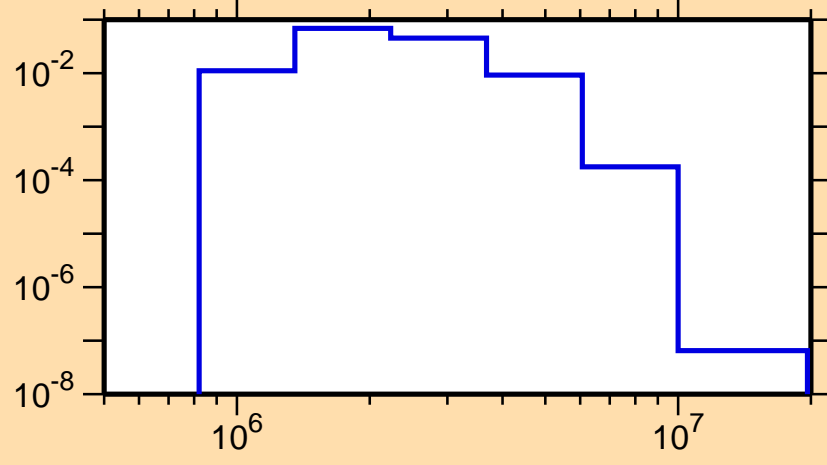
\sigma vs. E for ^{122}\text{Xe}(n,n_4)
