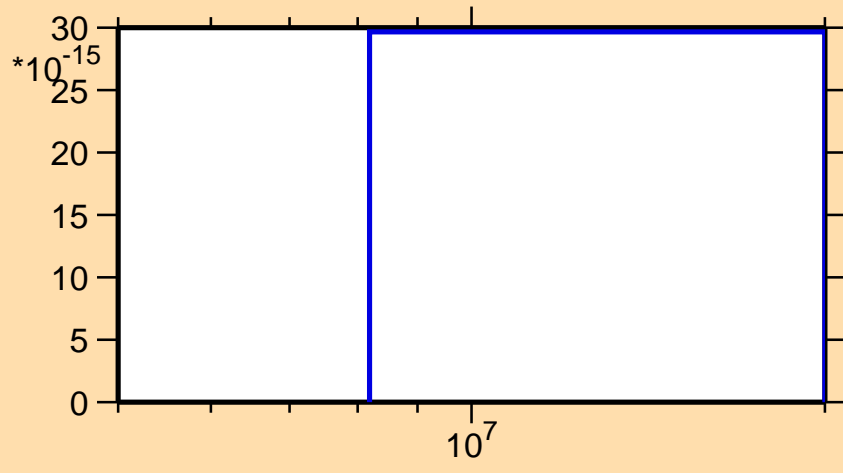
\sigma vs. E for ^{122}\text{Xe}(n,\text{pt})
