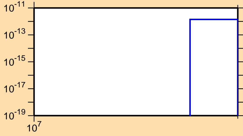
\sigma vs. E for ^{123}\text{Xe}(n,nt)
