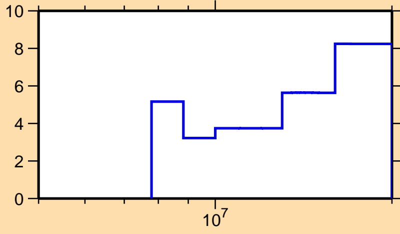
\Delta\sigma/\sigma vs. E for ^{123}\text{Xe}(n,\text{tot.})
