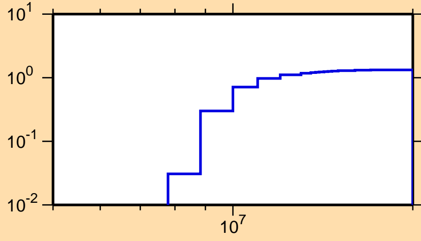
\sigma vs. E for ^{123}\text{Xe}(n,2n)
