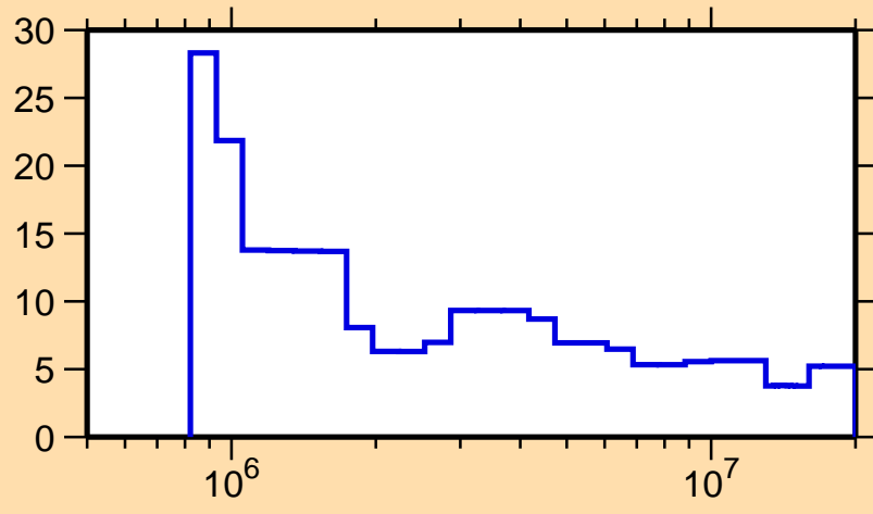
\Delta\sigma/\sigma vs. E for ^{123}\text{Xe}(n,\text{nonel.})
