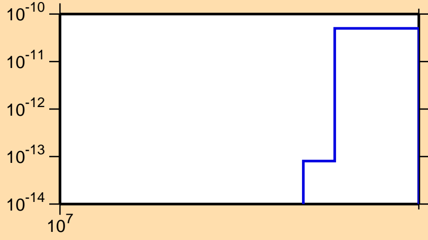
\sigma vs. E for ^{123}\text{Xe} (mt 34)
