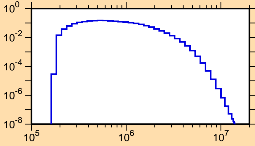
\sigma vs. E for ^{123}\text{Xe}(n,n_2)
