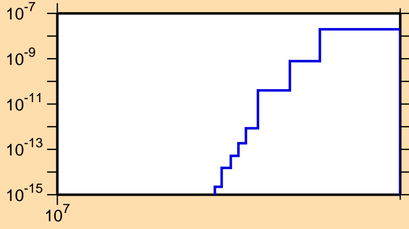
\sigma vs. E for ^{123}\text{Xe}(n,\text{pd})
