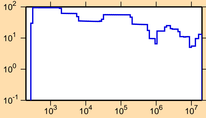
\Delta\sigma/\sigma vs. E for ^{123}\text{Xe}(n,el.)
