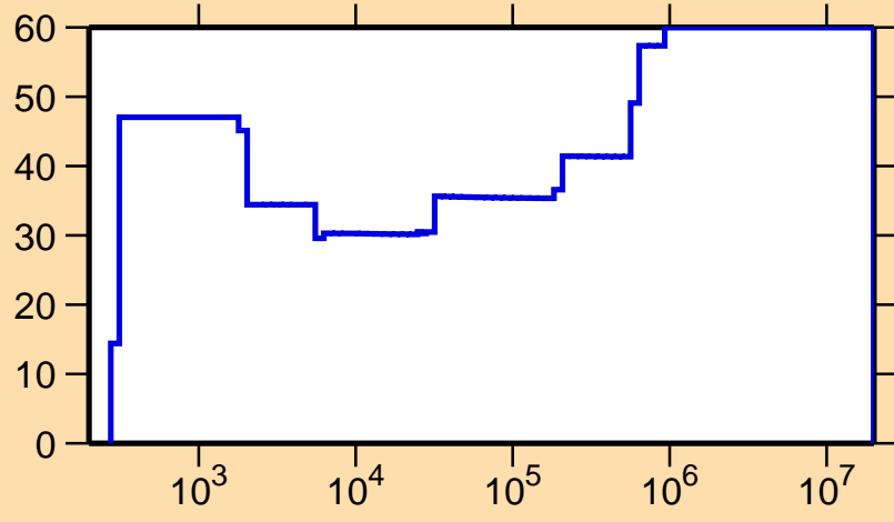
\Delta\sigma/\sigma vs. E for ^{123}\text{Xe}(n,p)
