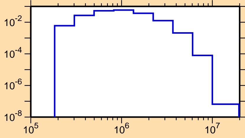
\sigma vs. E for ^{123}\text{Xe}(n,n_3)
