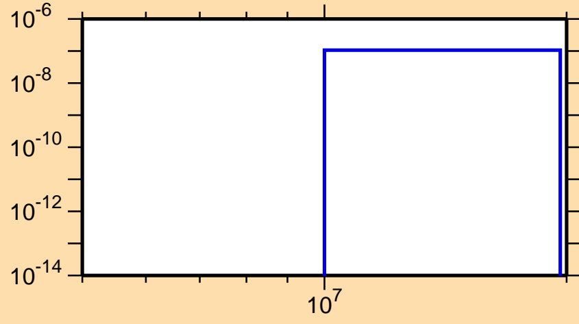
\sigma vs. E for ^{123}\text{Xe}(n,\text{He}3)
