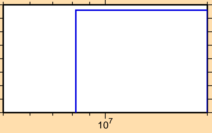
\sigma vs. E for ^{123}\text{Xe}(\text{mt117})
