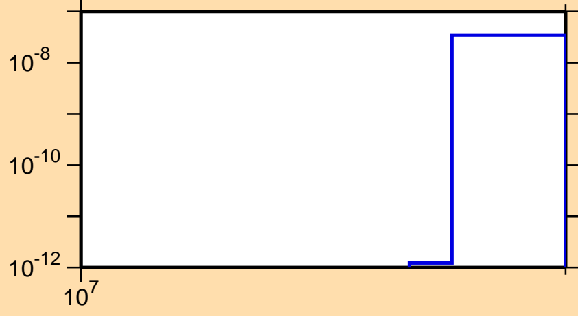
\sigma vs. E for ^{124}\text{Xe}(n,nd)
