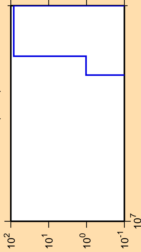
\Delta\sigma/\sigma vs. E for ^{124}\text{Xe}(n,nd)
