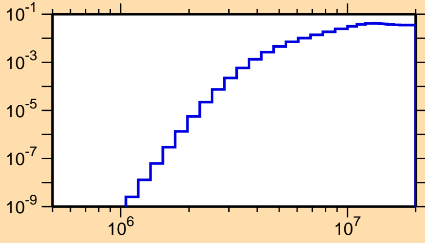
\sigma vs. E for ^{124}\text{Xe}(n,p)
