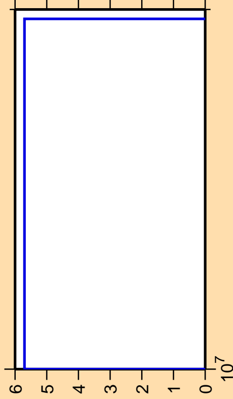
\Delta\sigma/\sigma vs. E for ^{124}\text{Xe}(\text{mt117})
