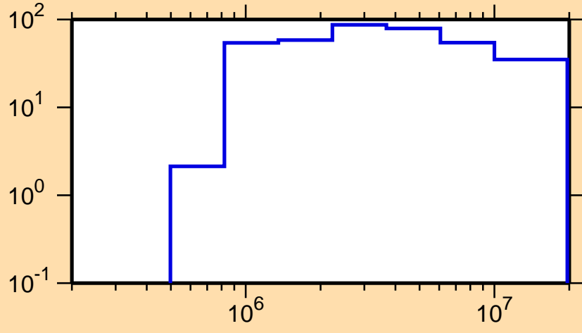
\Delta\sigma/\sigma vs. E for ^{124}\text{Xe}(n,p)
