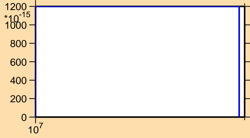
\sigma vs. E for ^{124}\text{Xe} (mt 45)
