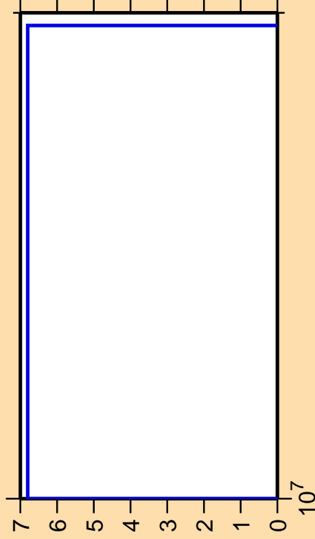
\Delta\sigma/\sigma vs. E for ^{124}\text{Xe} (mt 45)
