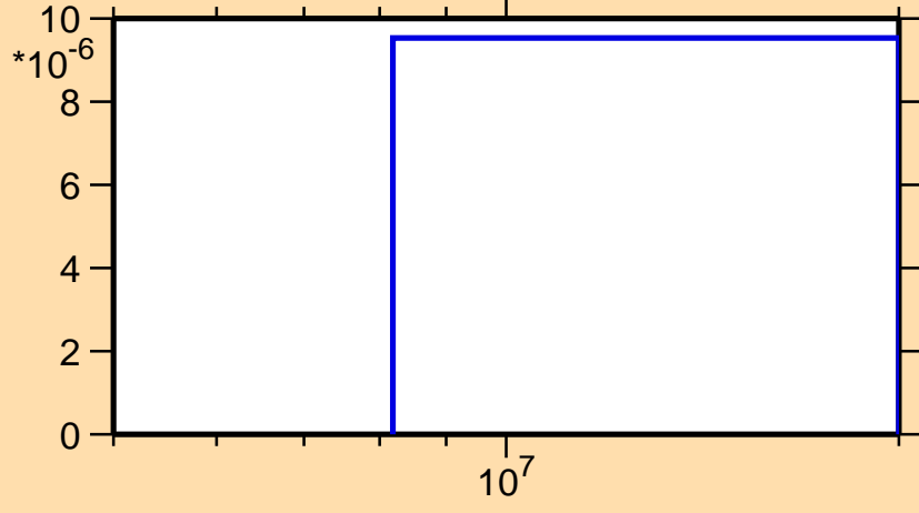
\sigma vs. E for ^{124}\text{Xe}(n,t)
