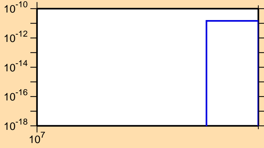
\sigma vs. E for ^{125}\text{Xe}(n,nt)
