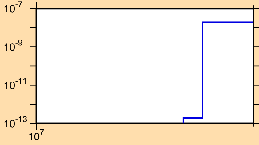
\sigma vs. E for ^{126}\text{Xe}(n,\text{nd})
