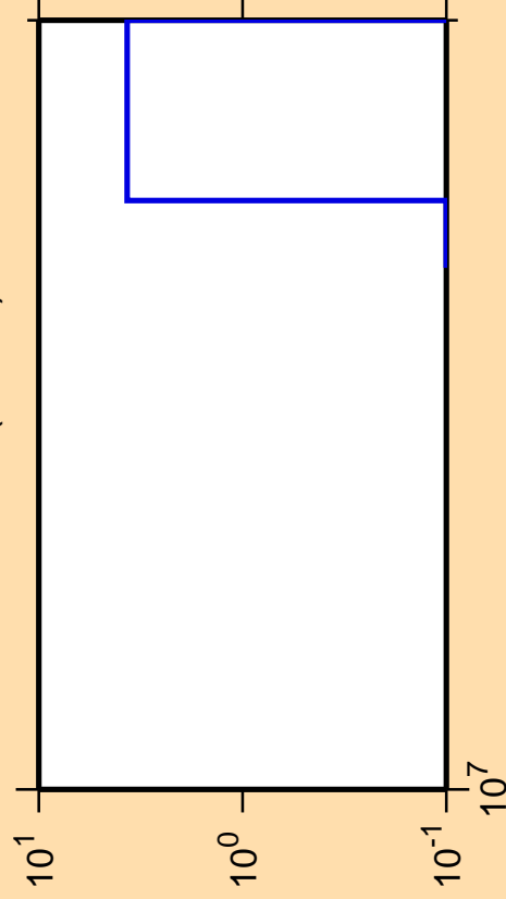
\Delta\sigma/\sigma vs. E for ^{126}\text{Xe}(\text{mt } 45)
