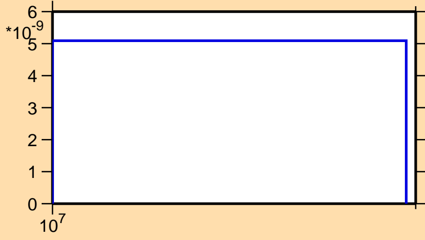
\sigma vs. E for ^{126}\text{Xe}(n,\text{He}3)
