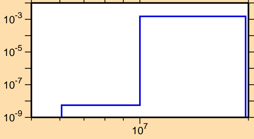
\sigma vs. E for ^{126}\text{Xe}(n,d)
