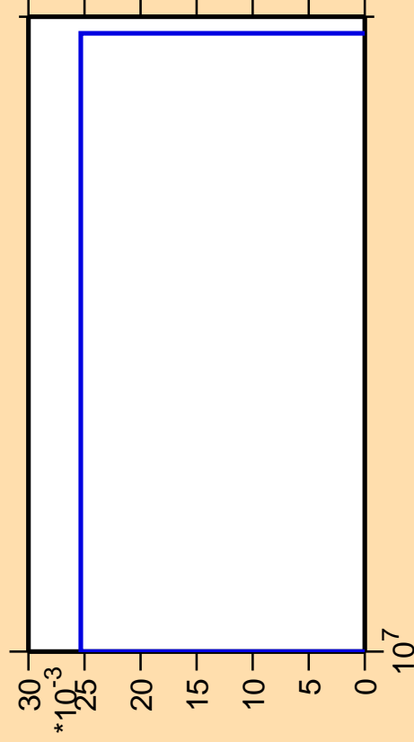
\Delta\sigma/\sigma vs. E for ^{126}\text{Xe}(\text{mt } 45)
