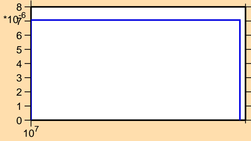
\sigma vs. E for ^{126}\text{Xe}(n,3n)
