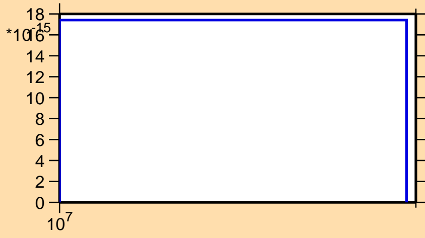
\sigma vs. E for ^{126}\text{Xe}(\text{mt117})
