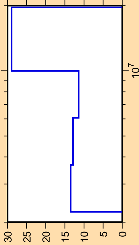
\Delta\sigma/\sigma vs. E for ^{126}\text{Xe}(n,n\text{cont.})
