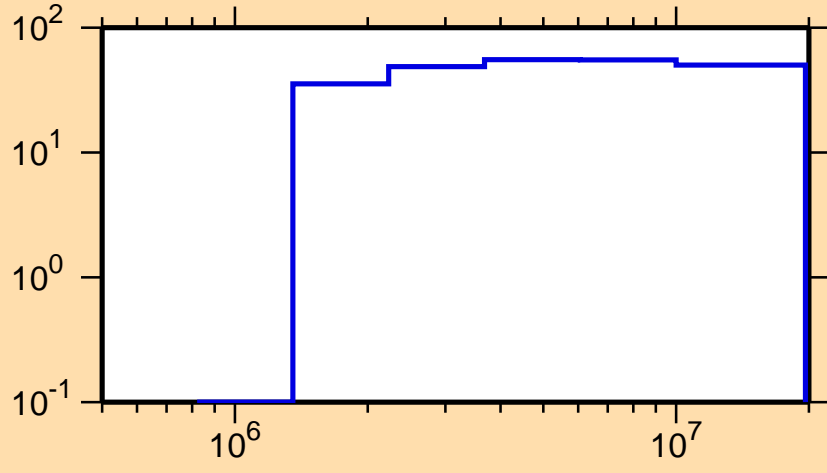
\Delta\sigma/\sigma vs. E for ^{126}\text{Xe}(n,p)
