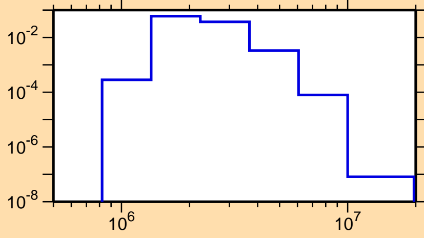
\sigma vs. E for ^{126}\text{Xe}(n,n_4)
