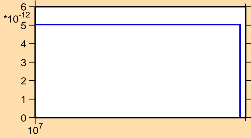
\sigma vs. E for ^{126}\text{Xe}(n,2np)
