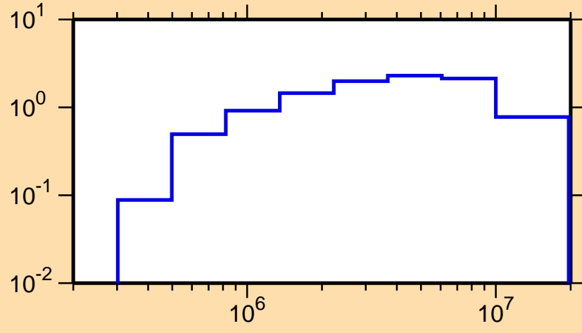
\sigma vs. E for ^{126}\text{Xe}(n,\text{inel.})
