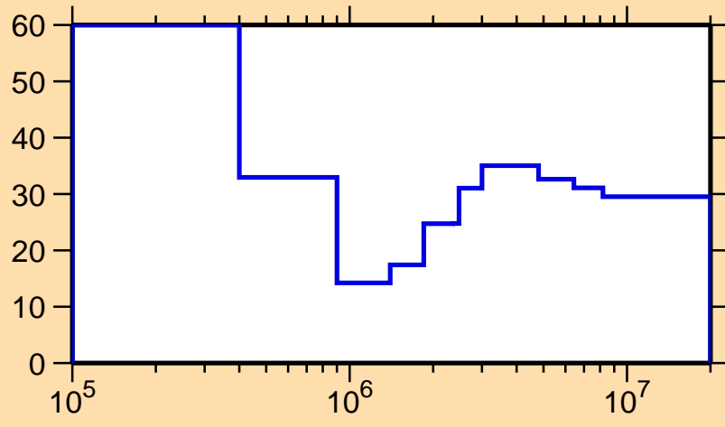
\Delta\sigma/\sigma vs. E for ^{126}\text{Xe}(n,n_1)
