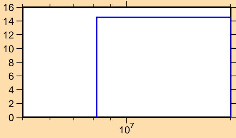
\Delta\sigma/\sigma vs. E for ^{126}\text{Xe}(n,\text{inel.})
