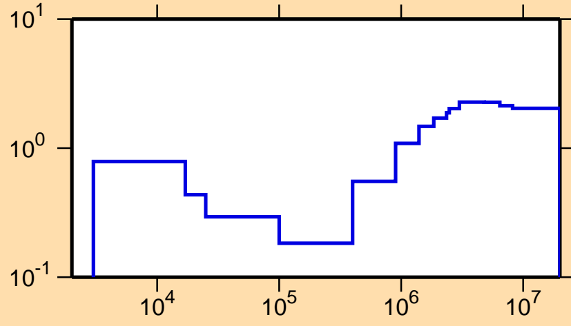
\sigma vs. E for ^{126}\text{Xe}(n,\text{nonel.})
