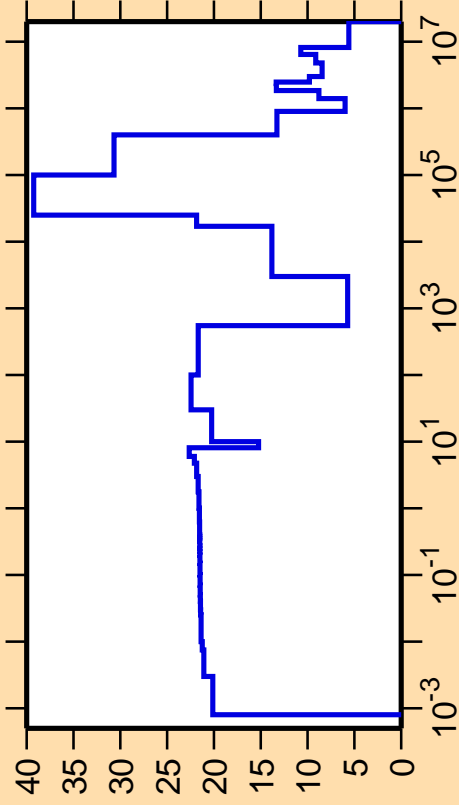
\Delta\sigma/\sigma vs. E for ^{126}\text{Xe}(n,\text{el.})
