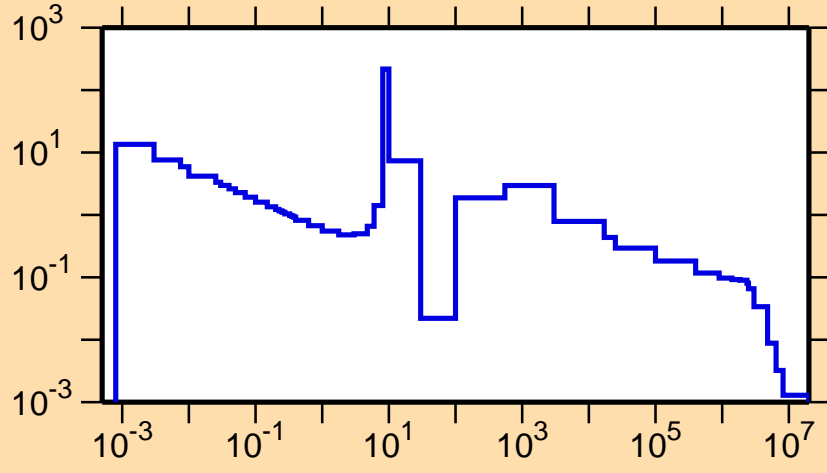
\sigma vs. E for ^{126}\text{Xe}(n,\gamma)
