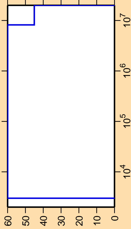
\Delta\sigma/\sigma vs. E for ^{126}\text{Xe}(n,\alpha)
