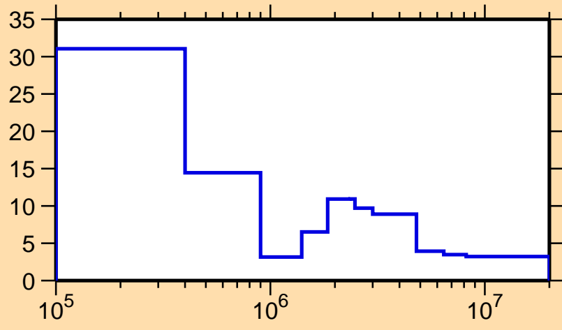
\Delta\sigma/\sigma vs. E for ^{126}\text{Xe}(n,\text{tot.})
