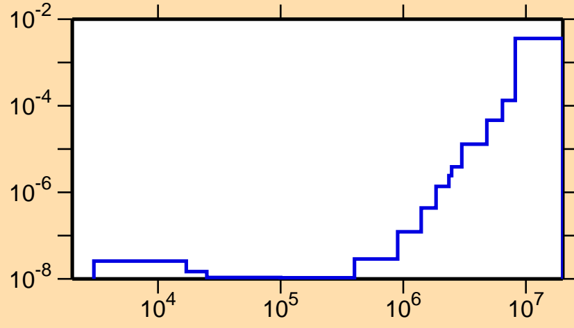
\sigma vs. E for ^{126}\text{Xe}(n,\alpha)
