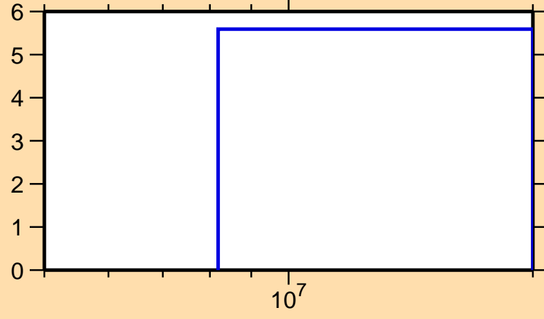
\Delta\sigma/\sigma vs. E for ^{126}\text{Xe}(n,\text{el.})
