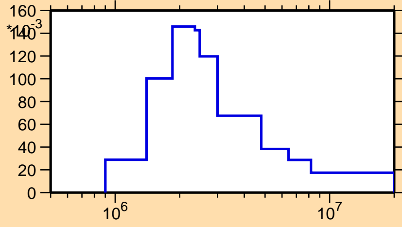
\sigma vs. E for ^{126}\text{Xe}(n,n_3)
