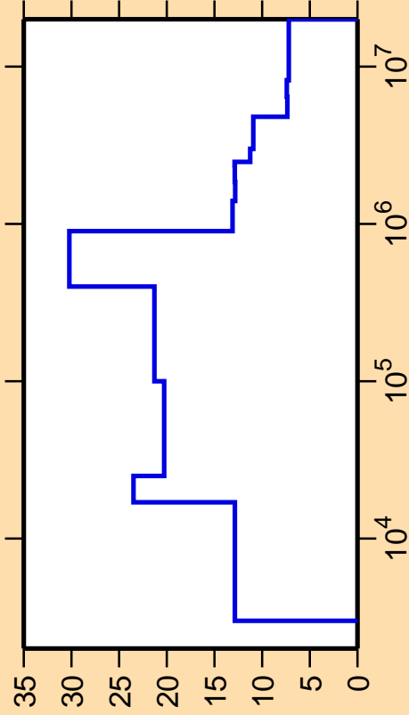
\Delta\sigma/\sigma vs. E for ^{126}\text{Xe}(n,\text{nonel.})
