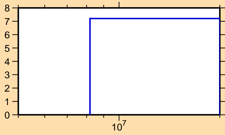
\Delta\sigma/\sigma vs. E for ^{126}\text{Xe}(n,\text{nonel.})
