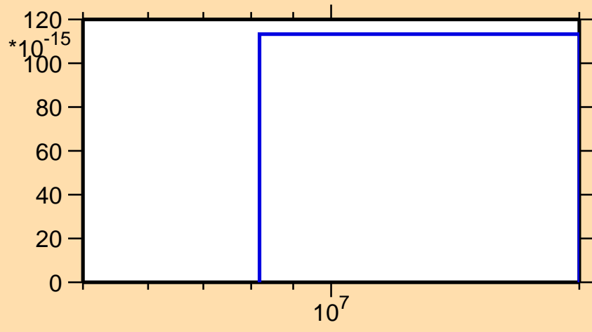
\sigma vs. E for ^{126}\text{Xe}(n,nt)
