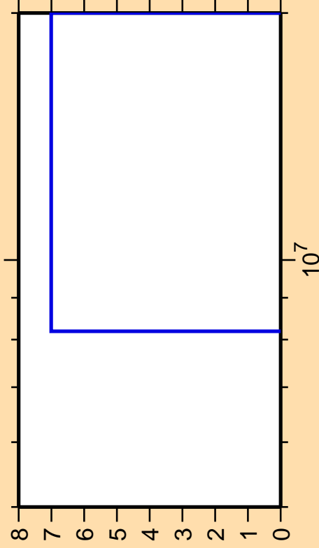
\Delta\sigma/\sigma vs. E for ^{126}\text{Xe}(n,pd)
