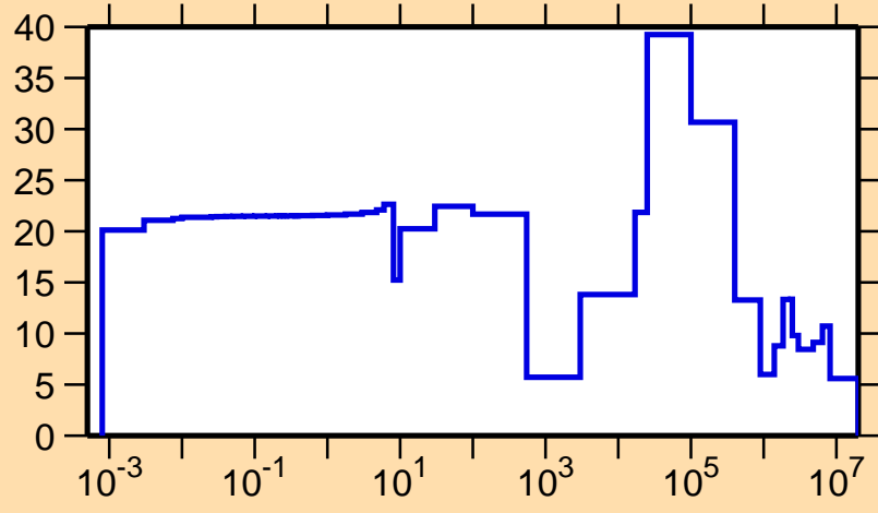
\Delta\sigma/\sigma vs. E for ^{126}\text{Xe}(n,\text{el.})
