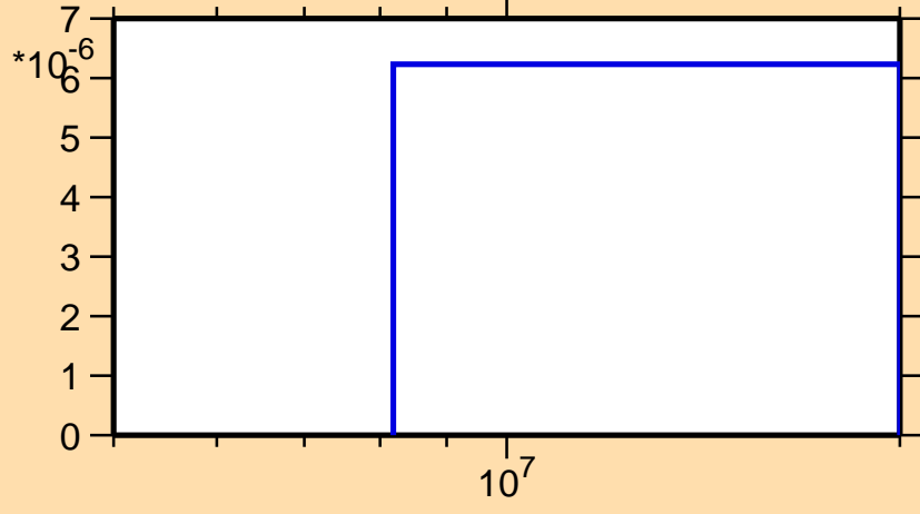
\sigma vs. E for ^{126}\text{Xe}(n,t)
