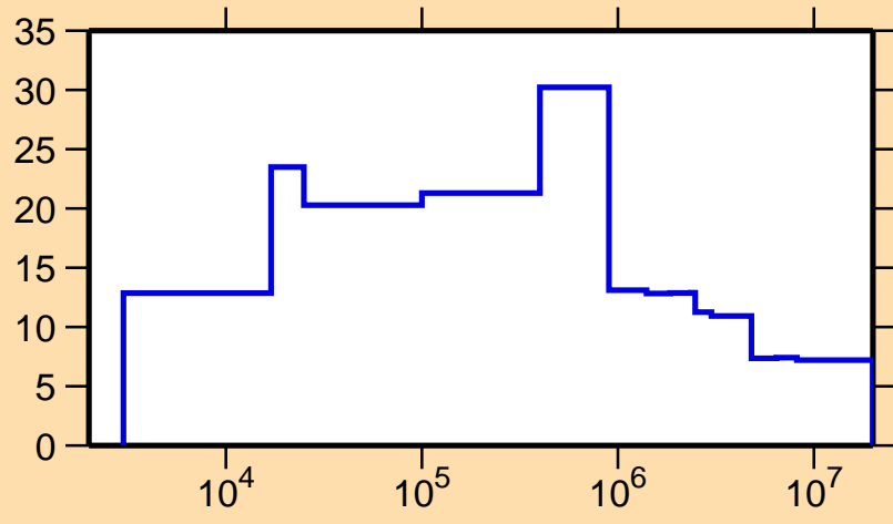
\Delta\sigma/\sigma vs. E for ^{126}\text{Xe}(n,\text{nonel.})
