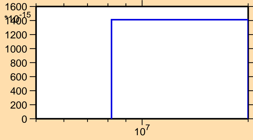
\sigma vs. E for ^{126}\text{Xe}(n,pd)
