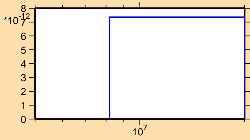
\sigma vs. E for ^{126}\text{Xe}(n,2np)
