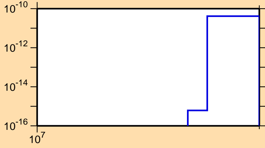
\sigma vs. E for ^{127}\text{Xe}(n,nt)
