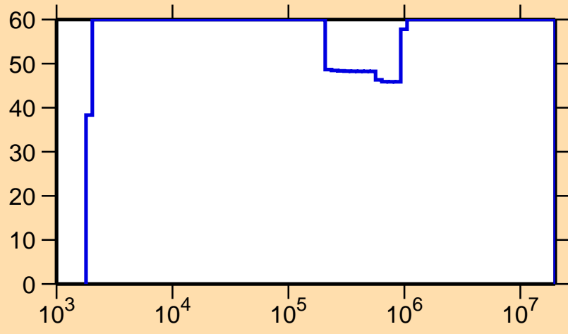
\Delta\sigma/\sigma vs. E for ^{127}\text{Xe}(n,p)
