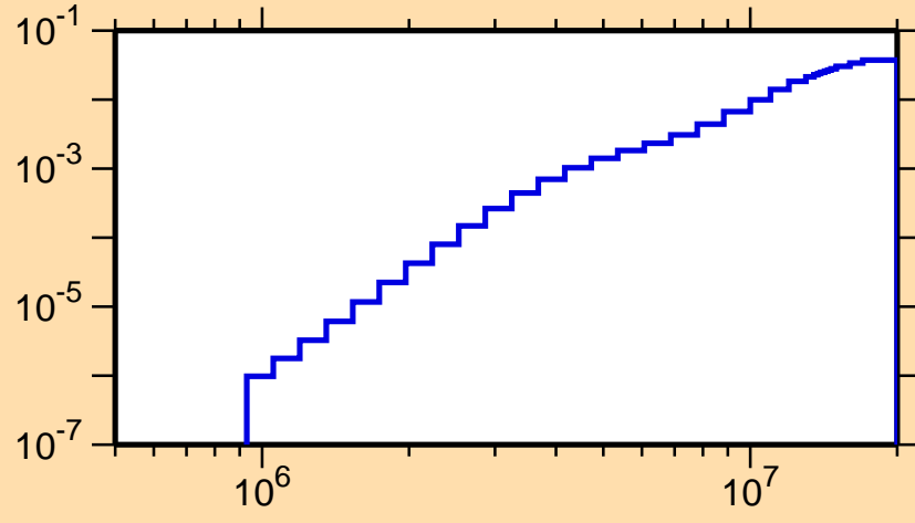
\sigma vs. E for ^{127}\text{Xe}(n,p)
