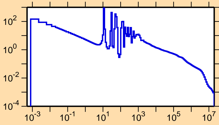
\sigma vs. E for ^{127}\text{Xe}(n,\gamma)
