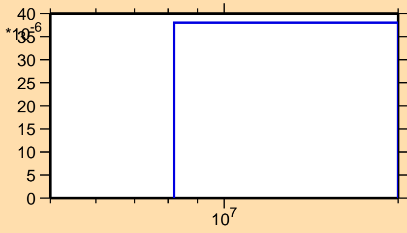
\sigma vs. E for ^{127}\text{Xe}(n,t)
