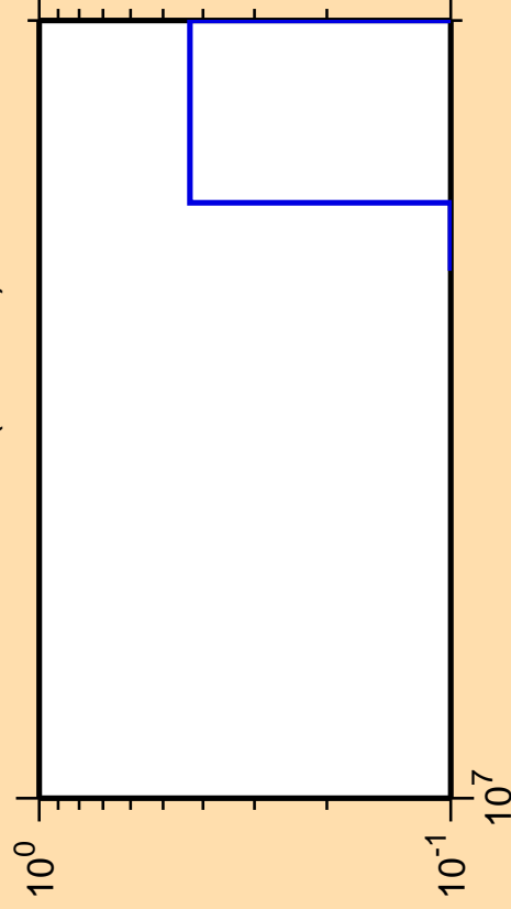
\Delta\sigma/\sigma vs. E for ^{127}\text{Xe}(\text{mt117})
