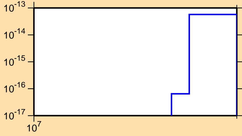
\sigma vs. E for ^{127}\text{Xe}(\text{mt117})
