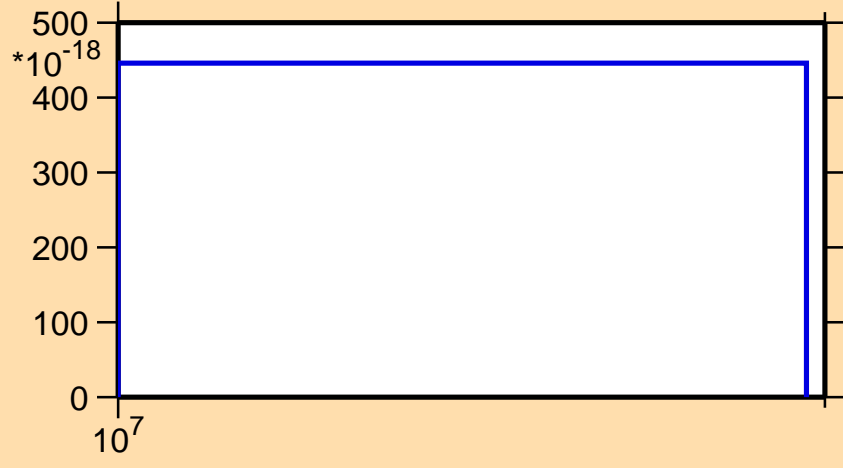
\sigma vs. E for ^{127}\text{Xe}(\text{mt117})
