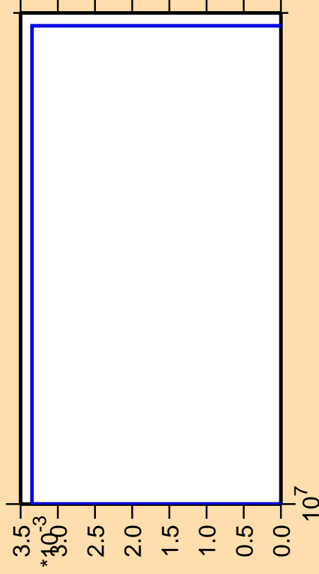
\Delta\sigma/\sigma vs. E for ^{127}\text{Xe}(\text{mt117})
