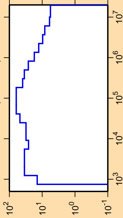
\Delta\sigma/\sigma vs. E for ^{127}\text{Xe}(n,\text{nonel.})
