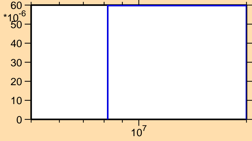
\sigma vs. E for ^{127}\text{Xe}(n,t)
