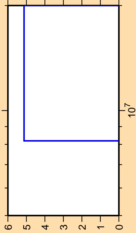
\Delta\sigma/\sigma vs. E for ^{127}\text{Xe}(n,nt)
