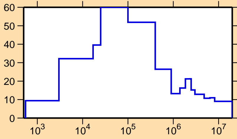
\Delta\sigma/\sigma vs. E for ^{127}\text{Xe}(n,el.)
