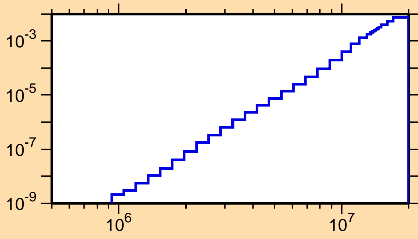
\sigma vs. E for ^{128}\text{Xe}(n,\alpha)
