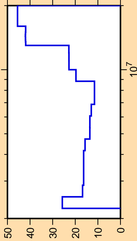
\Delta\sigma/\sigma vs. E for ^{128}\text{Xe}(n,\text{ncont.})
