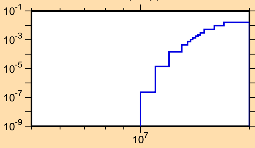
\sigma vs. E for ^{128}\text{Xe}(n,np)
