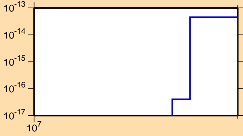
\sigma vs. E for ^{128}\text{Xe}(\text{mt117})
