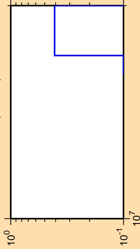
\Delta\sigma/\sigma vs. E for ^{128}\text{Xe}(\text{mt117})
