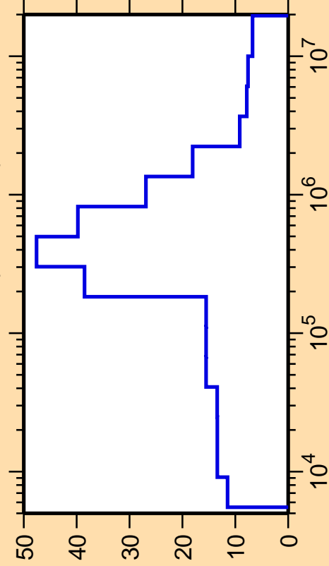
\Delta\sigma/\sigma vs. E for ^{128}\text{Xe}(n,\text{nonel.})
