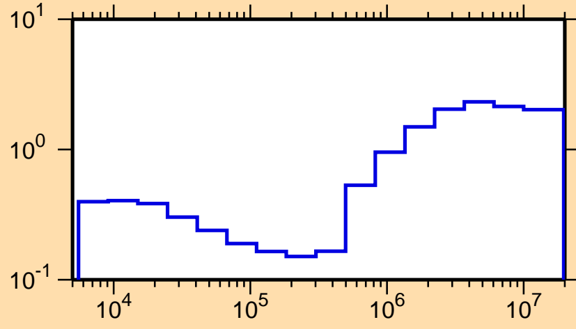
\sigma vs. E for ^{128}\text{Xe}(n,\text{nonel.})
