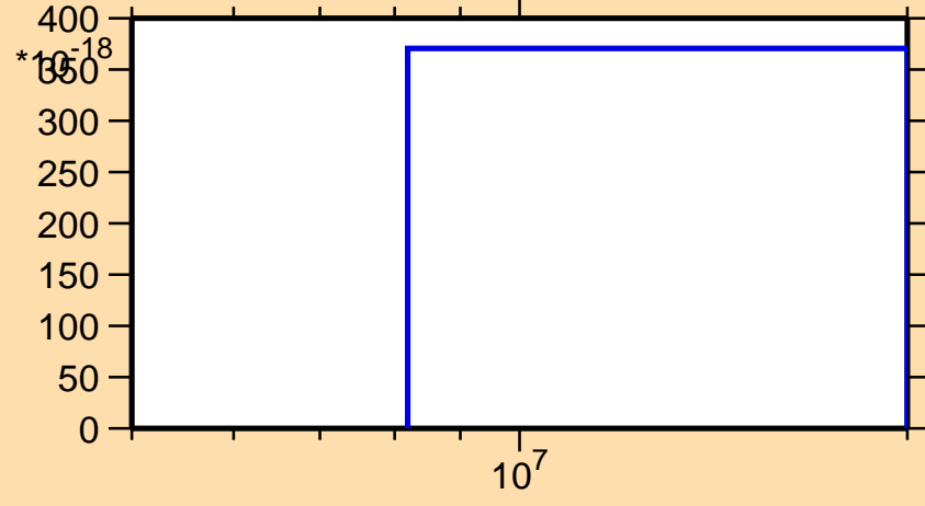
\sigma vs. E for ^{128}\text{Xe}(\text{mt117})
