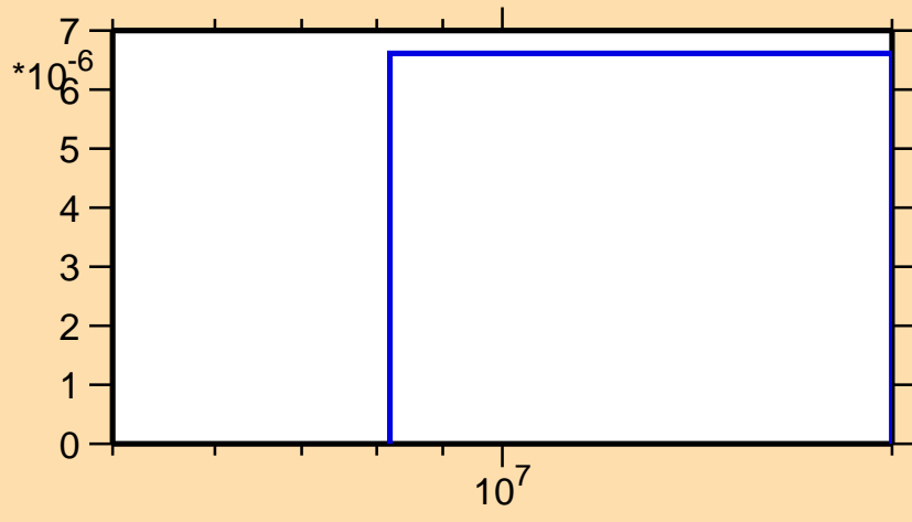
\sigma vs. E for ^{128}\text{Xe}(n,t)
