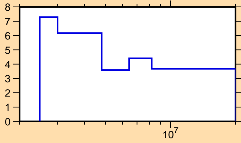
\Delta\sigma/\sigma vs. E for ^{128}\text{Xe}(n,\text{tot.})
