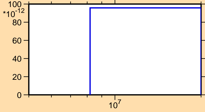
\sigma vs. E for ^{128}\text{Xe}(n,nd)
