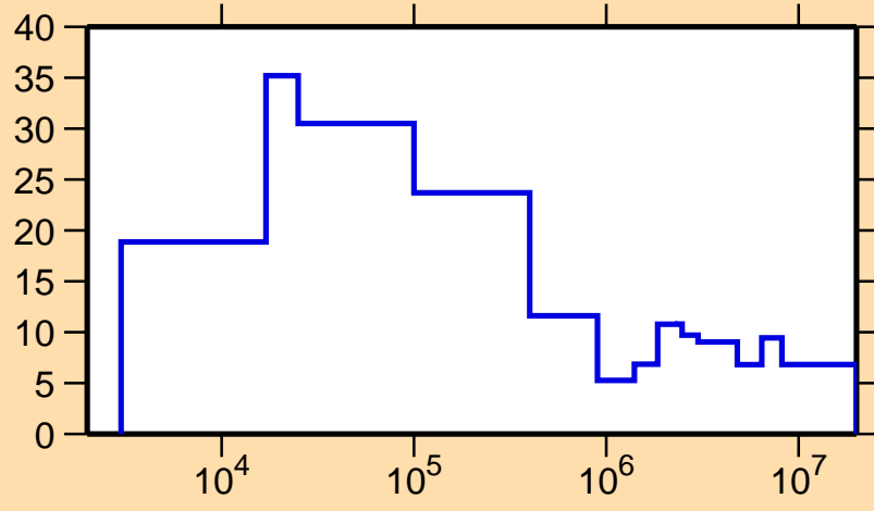
\Delta\sigma/\sigma vs. E for ^{128}\text{Xe}(n,\text{el.})
