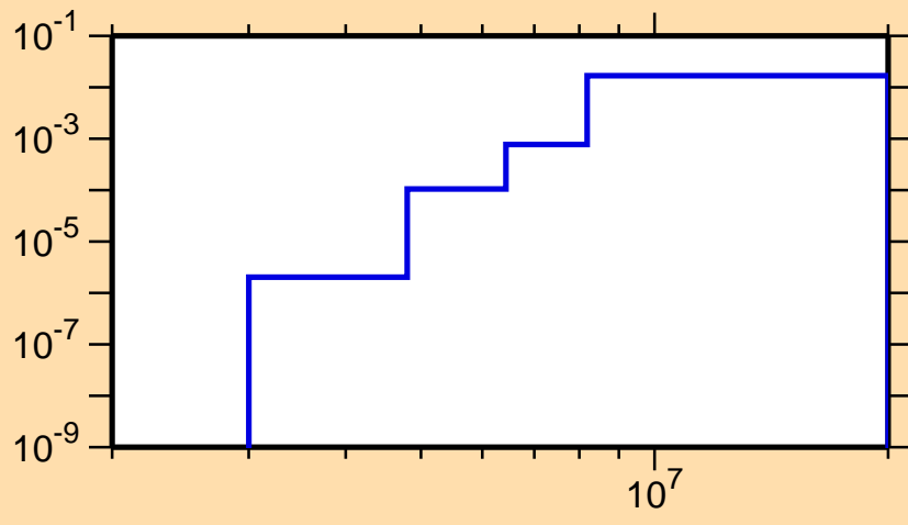
\sigma vs. E for ^{128}\text{Xe}(n,p)
