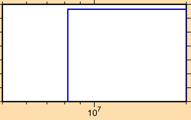
\sigma vs. E for ^{128}\text{Xe}(n,nt)
