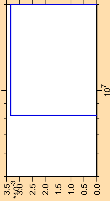
\Delta\sigma/\sigma vs. E for ^{128}\text{Xe}(\text{mt117})
