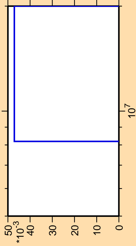
\Delta\sigma/\sigma vs. E for ^{128}\text{Xe}(n,\text{pd})
