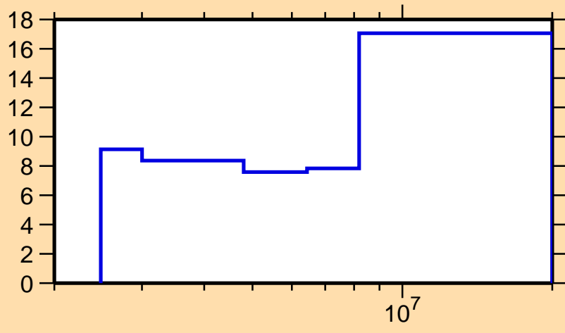
\Delta\sigma/\sigma vs. E for ^{128}\text{Xe}(n,\text{inel.})
