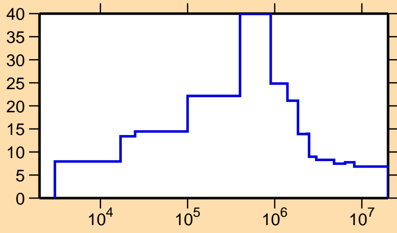
\Delta\sigma/\sigma vs. E for ^{128}\text{Xe}(n,\text{nonel.})
