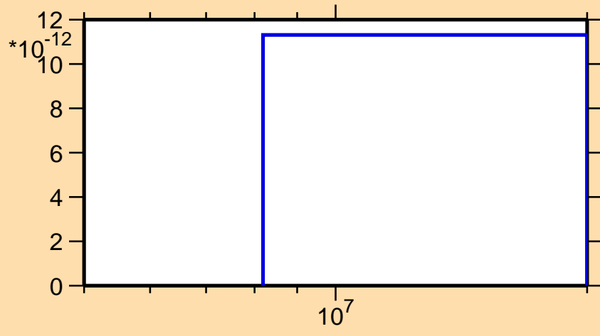
\sigma vs. E for ^{128}\text{Xe}(n,p\alpha)
