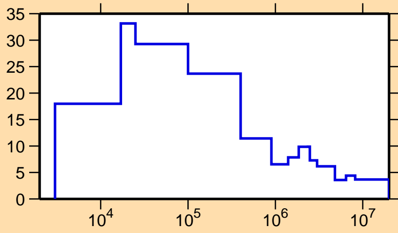
\Delta\sigma/\sigma vs. E for ^{128}\text{Xe}(n,\text{tot.})
