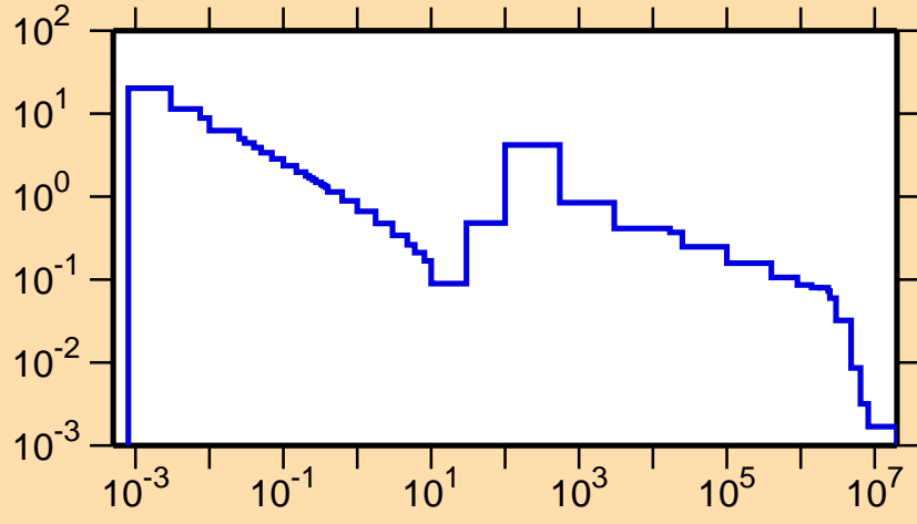
\sigma vs. E for ^{128}\text{Xe}(n,\gamma)
