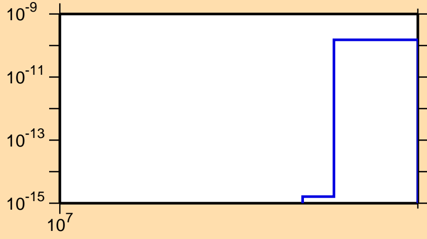
\sigma vs. E for ^{129}\text{Xe}(n,nt)
