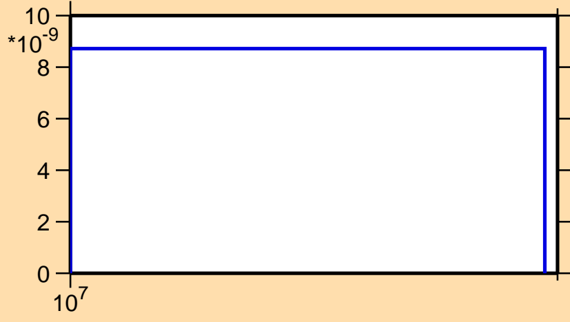
\sigma vs. E for ^{129}\text{Xe}(n,2n\alpha)
