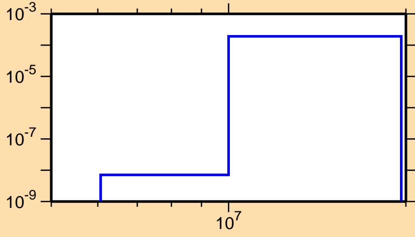
\sigma vs. E for ^{129}\text{Xe}(n,n\alpha)
