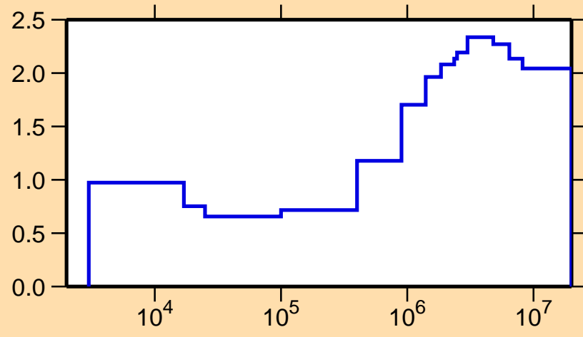
\sigma vs. E for ^{129}\text{Xe}(n,\text{nonel.})
