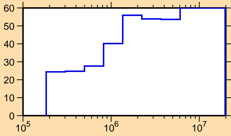
\Delta\sigma/\sigma vs. E for ^{129}\text{Xe}(n,\gamma)
