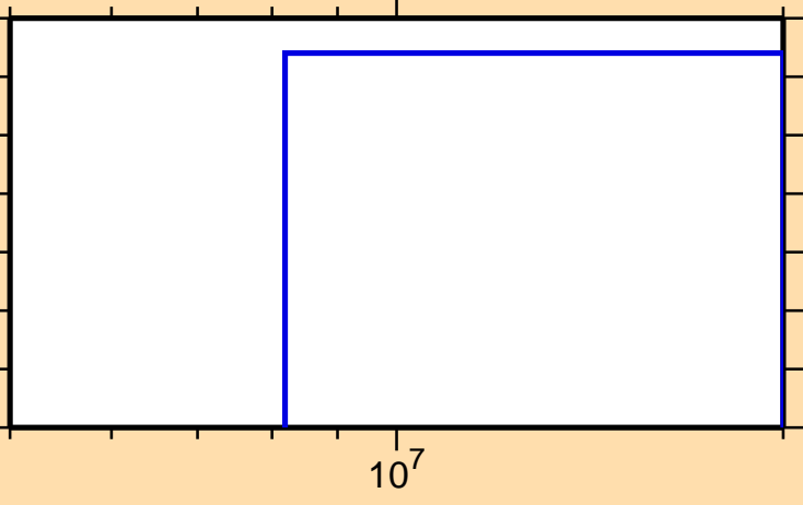
\sigma vs. E for ^{129}\text{Xe}(n,2np)
