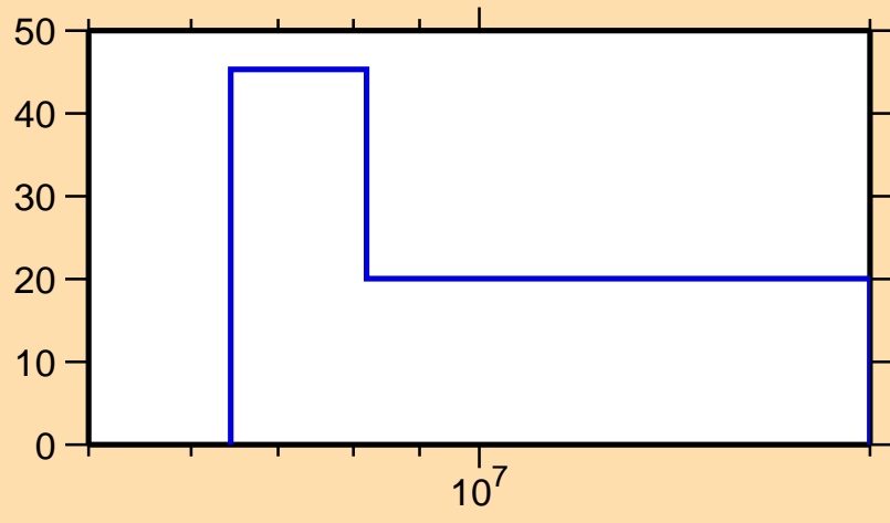
\Delta\sigma/\sigma vs. E for ^{129}\text{Xe}(n,2n)
