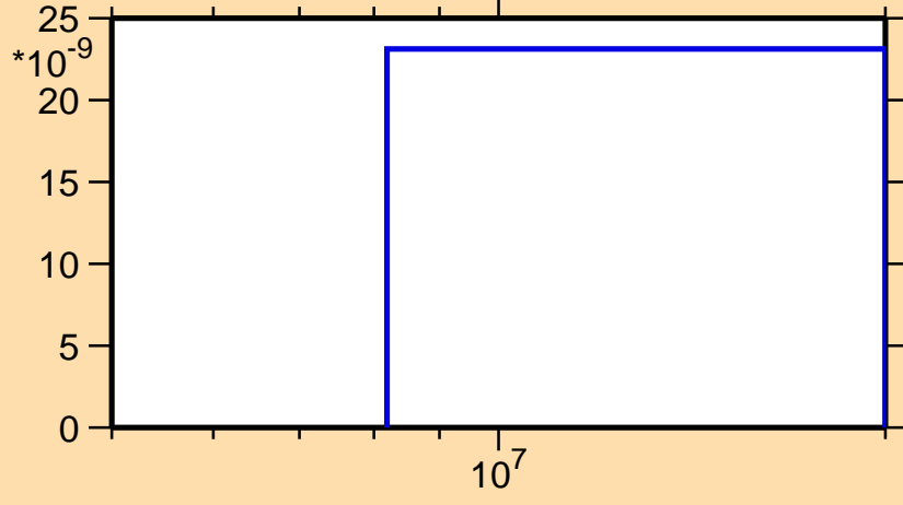
\sigma vs. E for ^{129}\text{Xe}(n,\text{nd})
