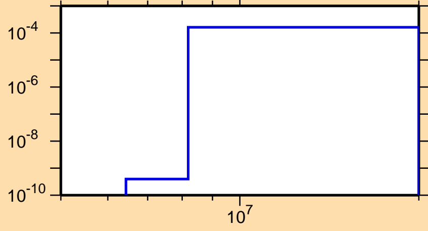
\sigma vs. E for ^{129}\text{Xe}(n,n\alpha)
