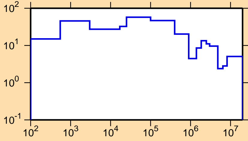
\Delta\sigma/\sigma vs. E for ^{129}\text{Xe}(n,\text{tot.})
