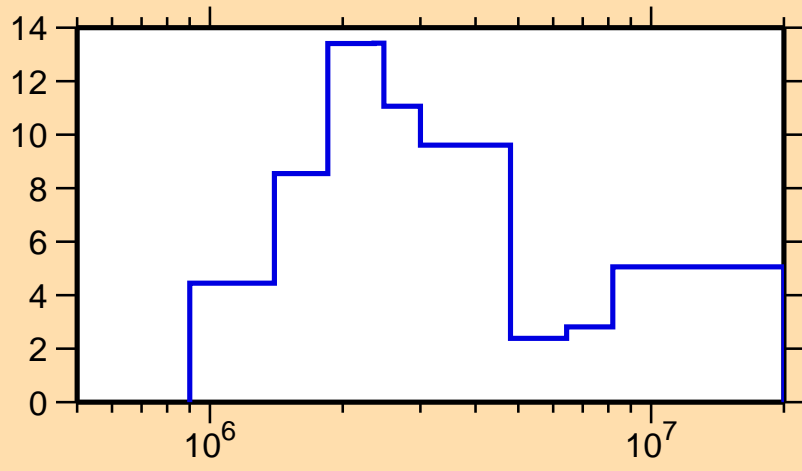
\Delta\sigma/\sigma vs. E for ^{129}\text{Xe}(n,\text{tot.})
