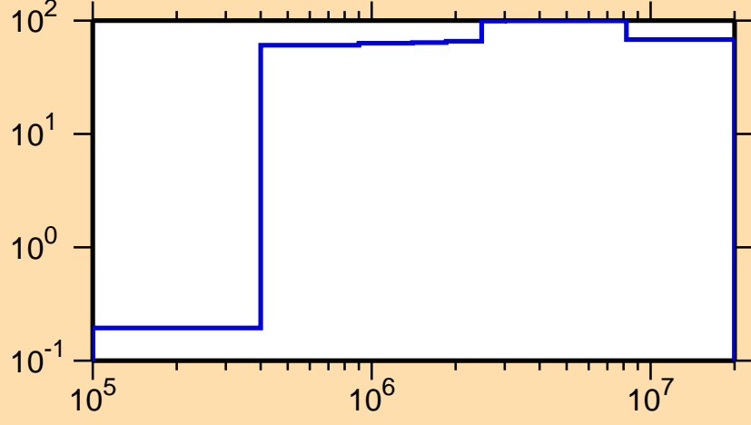
\Delta\sigma/\sigma vs. E for ^{129}\text{Xe}(n,p)
