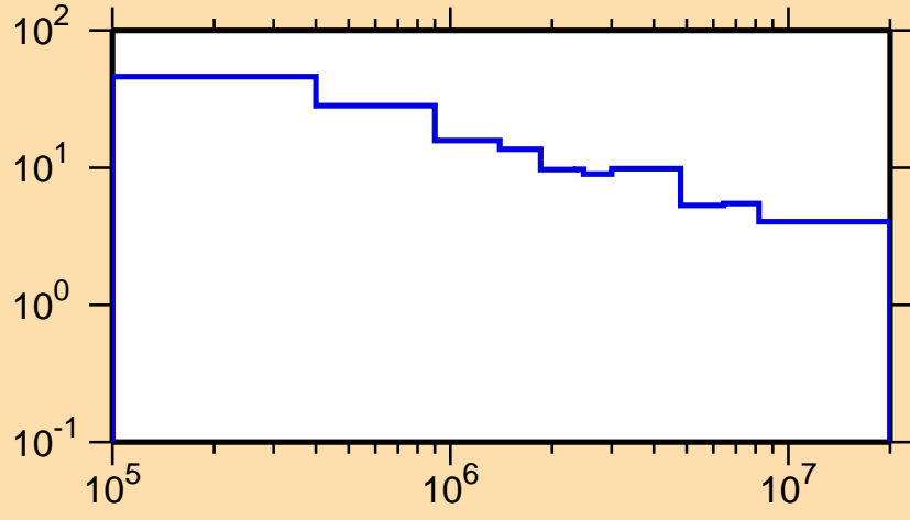
\Delta\sigma/\sigma vs. E for ^{129}\text{Xe}(n,\text{nonel.})
