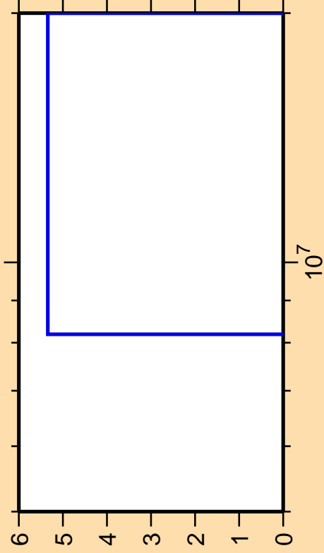
\Delta\sigma/\sigma vs. E for ^{129}\text{Xe}(n,nt)
