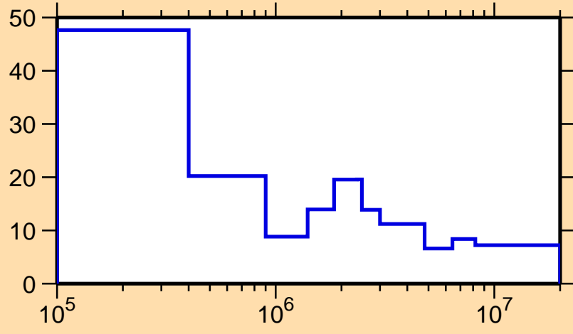
\Delta\sigma/\sigma vs. E for ^{129}\text{Xe}(n,\text{el.})
