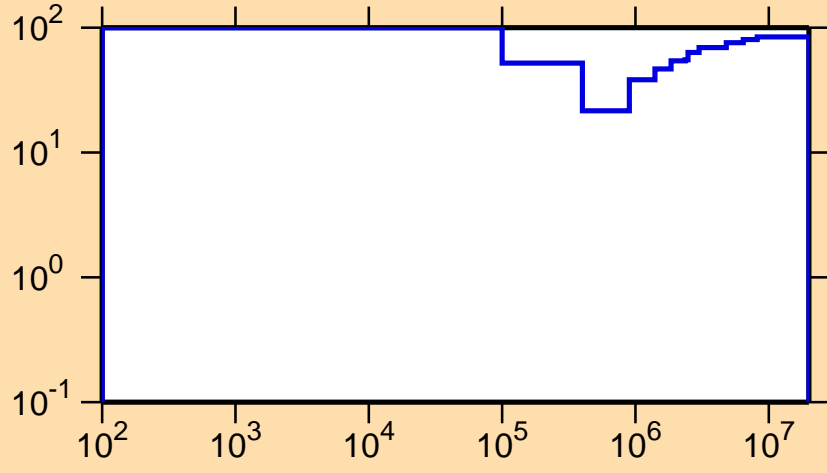
\Delta\sigma/\sigma vs. E for ^{129}\text{Xe}(n,n_1)
