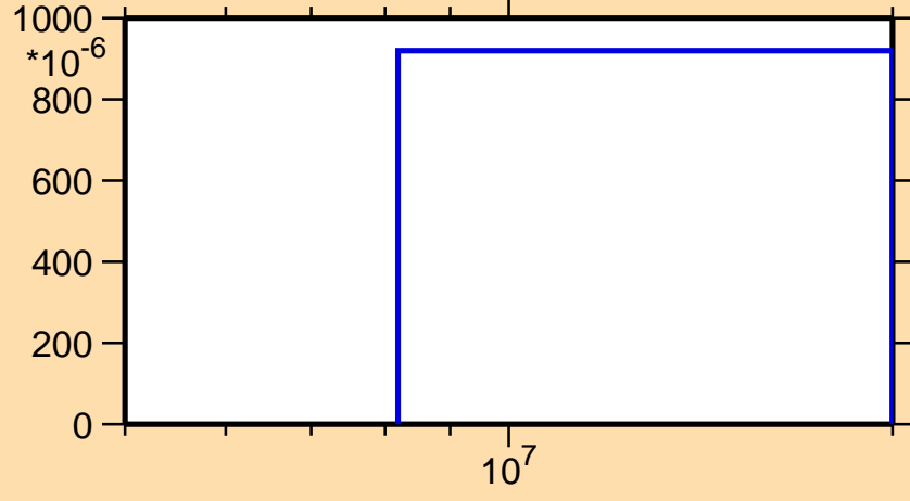
\sigma vs. E for ^{129}\text{Xe}(n,np)
