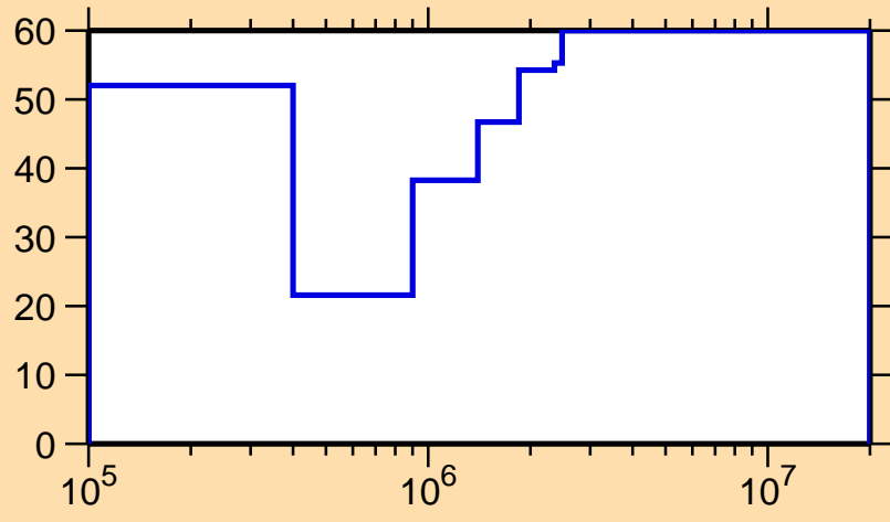
\Delta\sigma/\sigma vs. E for ^{129}\text{Xe}(n,n_1)
