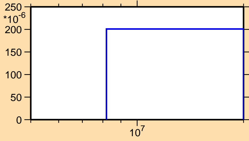
\sigma vs. E for ^{129}\text{Xe}(n,3n)
