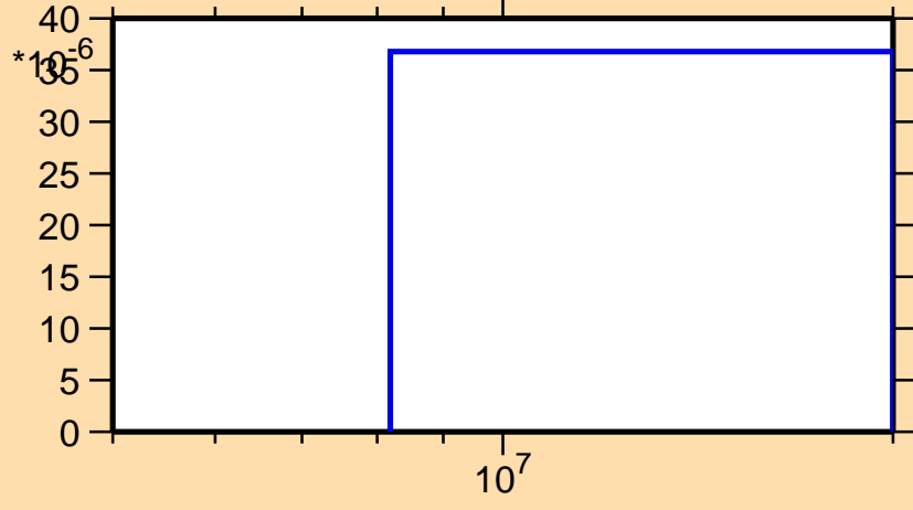
\sigma vs. E for ^{129}\text{Xe}(n,t)
