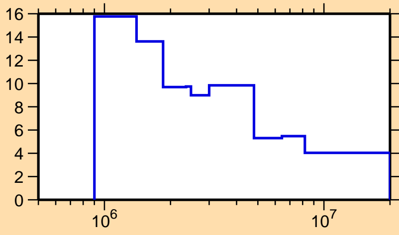
\Delta\sigma/\sigma vs. E for ^{129}\text{Xe}(n,\text{nonel.})
