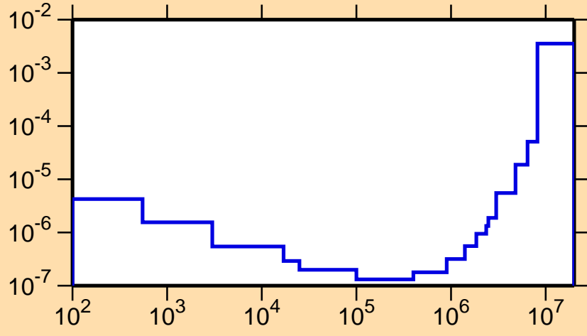
\sigma vs. E for ^{129}\text{Xe}(n,\alpha)
