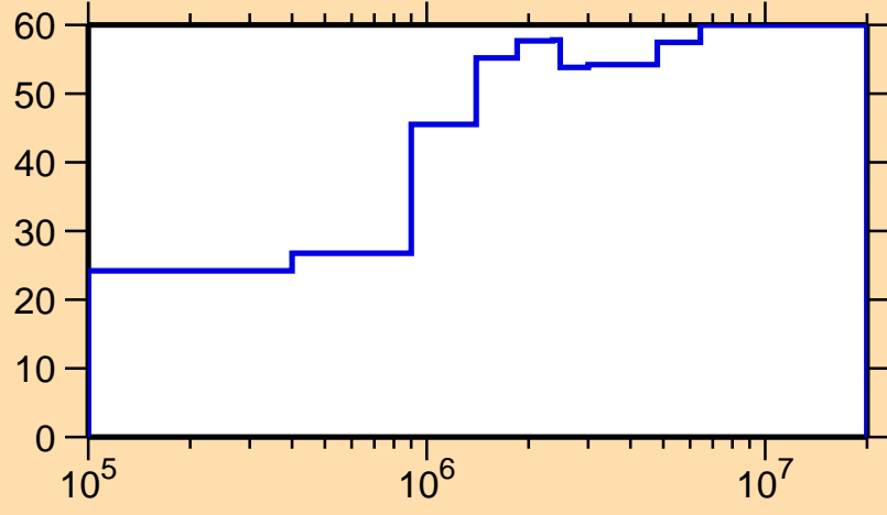
\Delta\sigma/\sigma vs. E for ^{129}\text{Xe}(n,\gamma)
