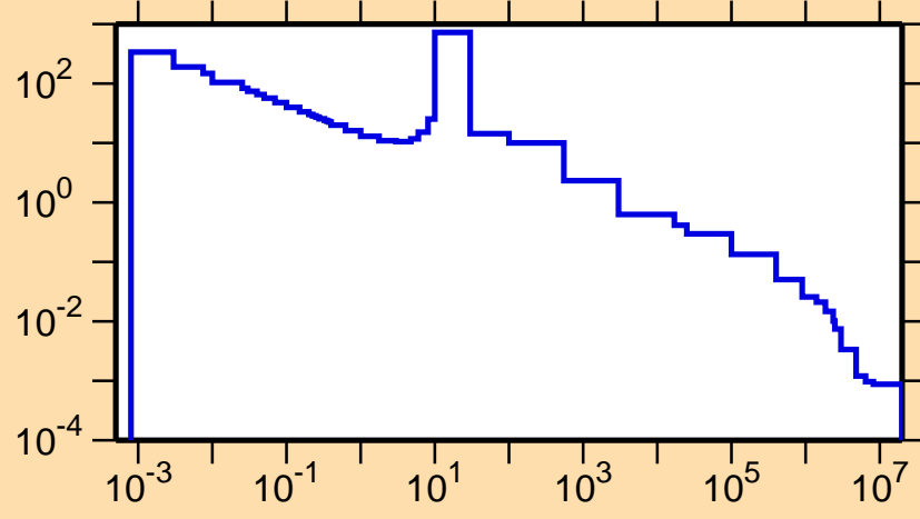
\sigma vs. E for ^{131}\text{Xe}(n,\gamma)
