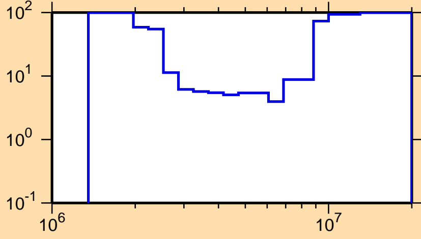
\Delta\sigma/\sigma vs. E for ^{131}\text{Xe}(n,n\text{cont.})
