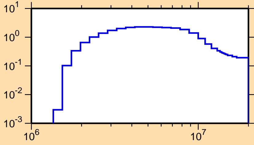
\sigma vs. E for ^{131}\text{Xe}(n,n\text{cont.})
